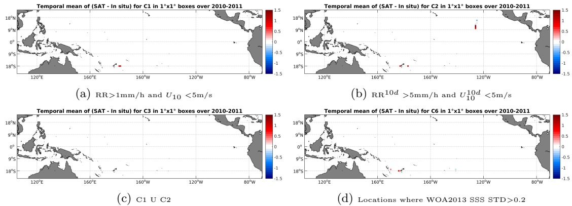
Figure 12: Temporal mean gridded over spatial boxes of size 1^\circ \times 1^\circ of \Delta SSS (SMOS-L3-CATDS-CECOS-IFREMER-V2-1DAY-0.5DEG - TSG-GOSUD-Sailing-ship) for 4 different subdatasets corresponding to: RR > 1 mm/h and U_{10} < 5 m/s (a), RR 10d > 5 mm/h and U_{10}^{10d} < 5 m/s (b), C1 U C2 (c), Locations where WOA2013 SSS STD > 0.2 (d).
