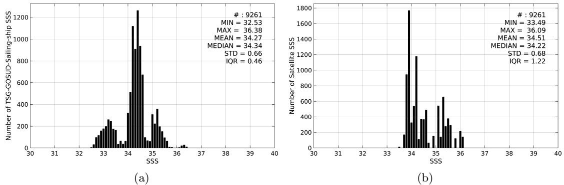
Figure 2: Histograms of SSS from TSG-GOSUD-Sailing-ship (a) and SMOS-L3-CATDS-CECOS-IFREMER-V2-1DAY-0.5DEG (b) considering all match-up pairs per bins of 0.1 over the Tropical Pacific Ocean Pi-MEP region and for the full satellite product period.
