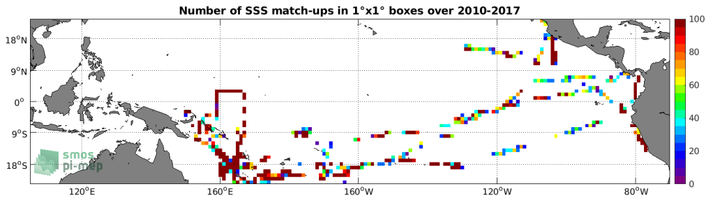
Figure 4: Number of SSS match-ups between TSG (GOSUD-Research-vessel) SSS and the SMOS SSS L3 v2 - Daily - 0.5 Deg (CATDS-CECOS-IFREMER) SSS product for the Tropical Pacific Ocean Pi-MEP region over 1°x1° boxes and for the full satellite product period.
