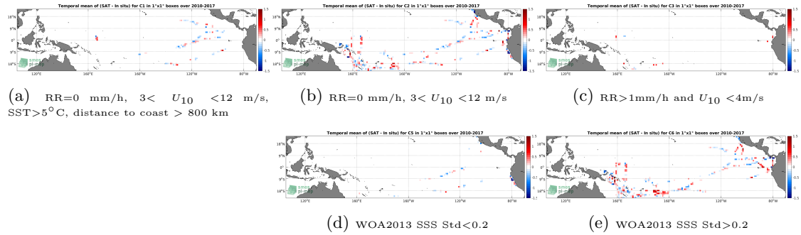
Figure 12: Temporal mean gridded over spatial boxes of size 1^{\circ}\times 1^{\circ} of \Delta SSS (SMOS SSS L3 v2 - Daily - 0.5 Deg (CATDS-CECOS-IFREMER) - TSG (GOSUD-Research-vessel)) for 5 different subdatasets corresponding to:RR=0 mm/h, 3 < U_{10} < 12 m/s, SST >5^{\circ}\text{C} , distance to coast > 800 km (a), RR=0 mm/h, 3 < U_{10} < 12 m/s (b), RR >1 mm/h and U_{10} < 4 m/s (c), WOA2013 SSS Std <0.2 (d), WOA2013 SSS Std >0.2 (e).
