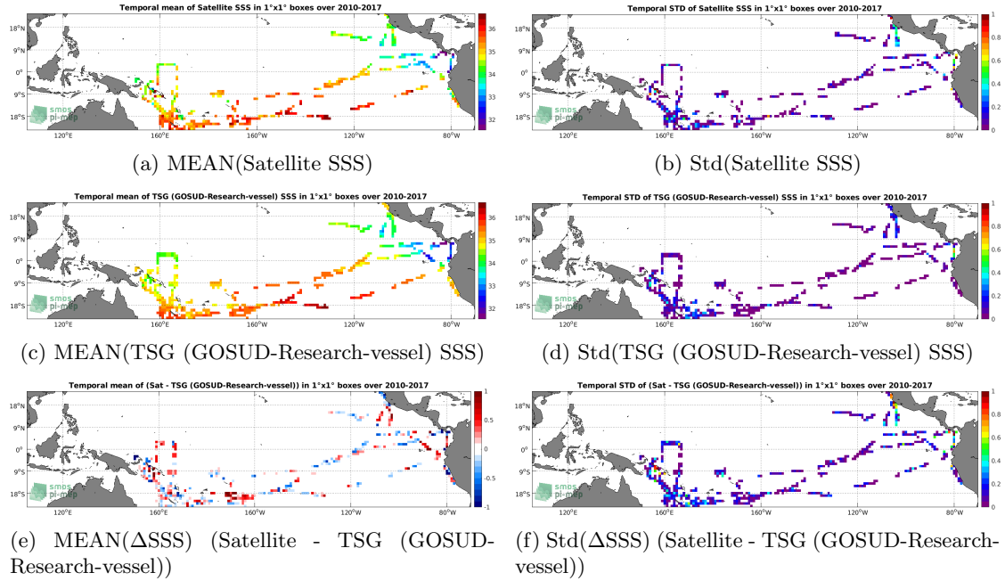
Figure 6: Temporal mean (left) and Std (right) of SSS from SMOS SSS L3 v2 - Daily - 0.5 Deg (CATDS-CECOS-IFREMER) (top), TSG (GOSUD-Research-vessel) (middle), and of \Delta SSS (Satellite - TSG (GOSUD-Research-vessel)). Only match-up pairs are used to generate these maps.
