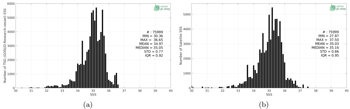
Figure 2: Histograms of SSS from TSG (GOSUD-Research-vessel) (a) and SMOS SSS L3 v2 - Daily - 0.5 Deg (CATDS-CECOS-IFREMER) (b) considering all match-up pairs per bins of 0.1 over the Tropical Pacific Ocean Pi-MEP region and for the full satellite product period.
