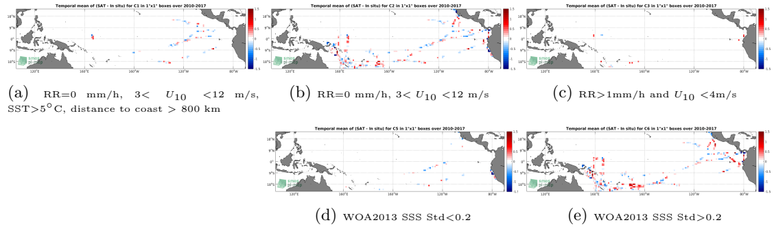
Figure 12: Temporal mean gridded over spatial boxes of size 1^{\circ}\times 1^{\circ} of \Delta SSS (SMOS SSS L3 v2 - Daily - 0.5 Deg (CATDS-CECOS-IFREMER) - TSG (GOSUD-Research-vessel)) for 5 different subdatasets corresponding to:RR=0 mm/h, 3 < U_{10} < 12 m/s, SST > 5^{\circ}\text{C} , distance to coast > 800 km (a), RR=0 mm/h, 3 < U_{10} < 12 m/s (b), RR > 1 mm/h and U_{10} < 4 m/s (c), WOA2013 SSS Std < 0.2 (d), WOA2013 SSS Std > 0.2 (e).
