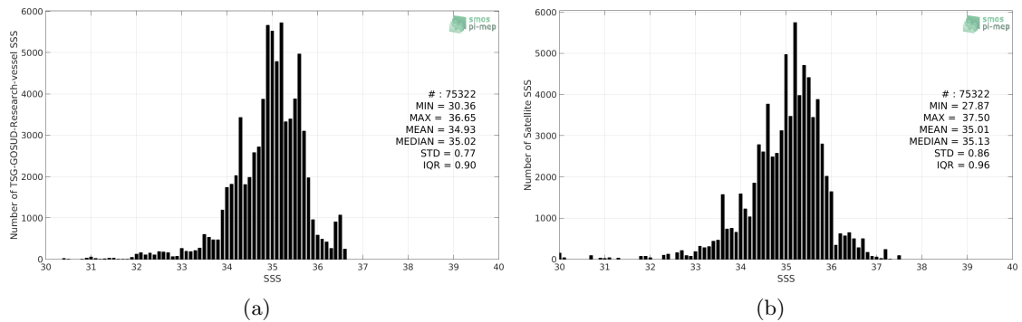
Figure 2: Histograms of SSS from TSG-GOSUD-Research-vessel (a) and SMOS L3 v2 - Daily - 0.5 Deg (CATDS-CECOS-IFREMER) (b) considering all match-up pairs per bins of 0.1 over the Tropical Pacific Ocean Pi-MEP region and for the full satellite product period.
