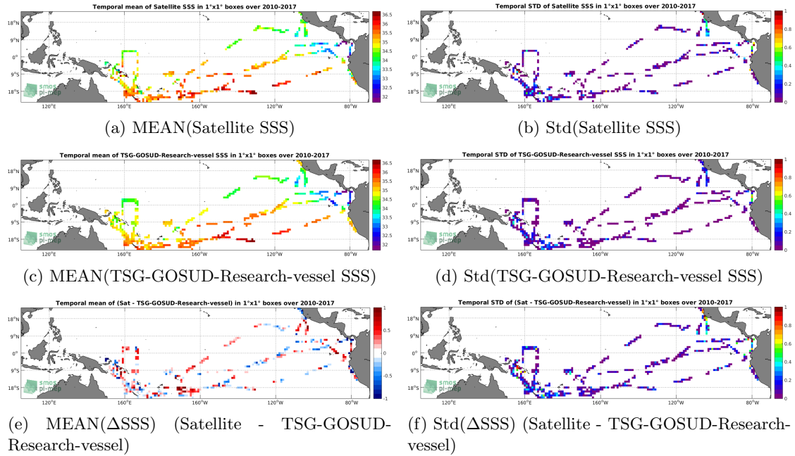
Figure 6: Temporal mean (left) and Std (right) of SSS from SMOS L3 v2 - Daily - 0.5 Deg (CATDS-CECOS-IFREMER) (top), TSG-GOSUD-Research-vessel (middle), and of \Delta SSS (Satellite - TSG-GOSUD-Research-vessel). Only match-up pairs are used to generate these maps.
