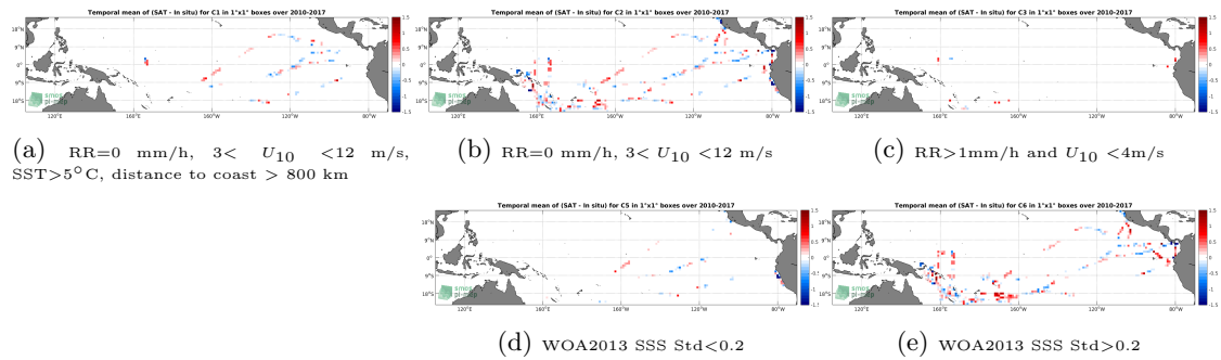
Figure 12: Temporal mean gridded over spatial boxes of size 1^{\circ}\times 1^{\circ} of \Delta SSS (SMOS L3 v2 - Daily - 0.5 Deg (CATDS-CECOS-IFREMER) - TSG-GOSUD-Research-vessel) for 5 different subdatasets corresponding to:RR=0 mm/h, 3 < U_{10} < 12 m/s, SST >5^{\circ}\text{C} , distance to coast > 800 km (a), RR=0 mm/h, 3 < U_{10} < 12 m/s (b), RR >1 mm/h and U_{10} < 4 m/s (c), WOA2013 SSS Std <0.2 (d), WOA2013 SSS Std >0.2 (e).
