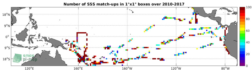
Figure 4: Number of SSS match-ups between TSG-GOSUD-Research-vessel SSS and the SMOS L3 v2 - Daily - 0.5 Deg (CATDS-CECOS-IFREMER) SSS product for the Tropical Pacific Ocean Pi-MEP region over 1°x1° boxes and for the full satellite product period.
