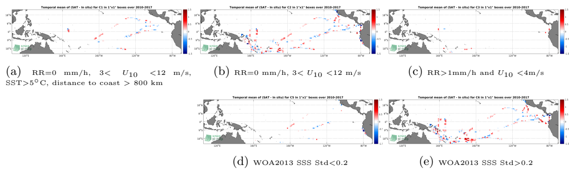
Figure 12: Temporal mean gridded over spatial boxes of size 1^\circ \times 1^\circ of \Delta SSS (SMOS-L3-CATDS-CECOS-IFREMER-V2-1DAY-0.5DEG - TSG-GOSUD-Research-vessel) for 5 different subdatasets corresponding to: RR=0 mm/h, 3 < U_{10} < 12 m/s, SST > 5°C, distance to coast > 800 km (a), RR=0 mm/h, 3 < U_{10} < 12 m/s (b), RR > 1mm/h and U_{10} < 4 m/s (c), WOA2013 SSS Std < 0.2 (d), WOA2013 SSS Std > 0.2 (e).
