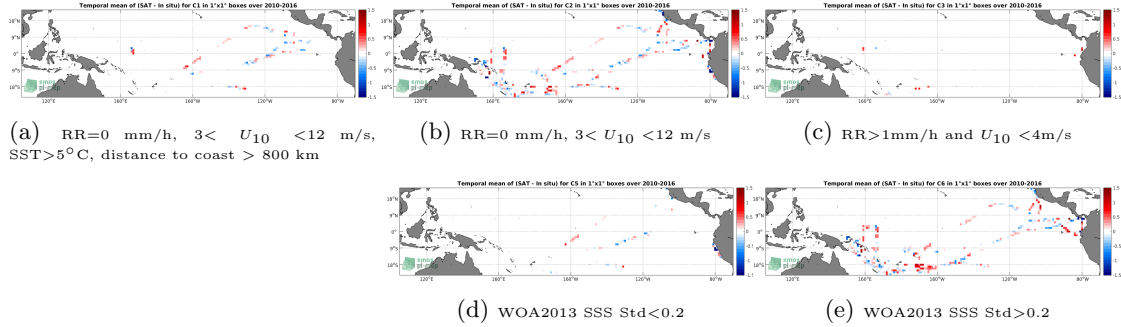
Figure 12: Temporal mean gridded over spatial boxes of size 1^\circ \times 1^\circ of \Delta SSS (SMOS-L3-CATDS-CECOS-IFREMER-V2-1DAY-0.5DEG - TSG-GOSUD-Research-vessel) for 5 different subdatasets corresponding to:RR=0 mm/h, 3 < U_{10} < 12 m/s, SST > 5^\circ C , distance to coast > 800 km (a), RR=0 mm/h, 3 < U_{10} < 12 m/s (b), RR >1 mm/h and U_{10} < 4 m/s (c), WOA2013 SSS Std <0.2 (d), WOA2013 SSS Std >0.2 (e).
