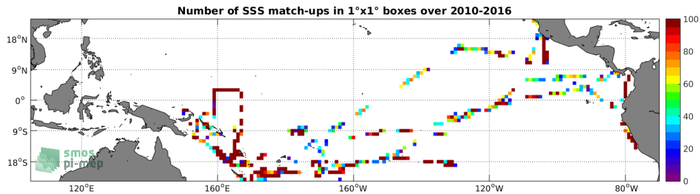
Figure 4: Number of SSS match-ups between TSG-GOSUD-Research-vessel SSS and the SMOS-L3-CATDS-CECOS-IFREMER-V2-1DAY-0.5DEG SSS product for the Tropical Pacific Ocean Pi-MEP region over 1^{\circ} \times 1^{\circ} boxes and for the full satellite product period.
