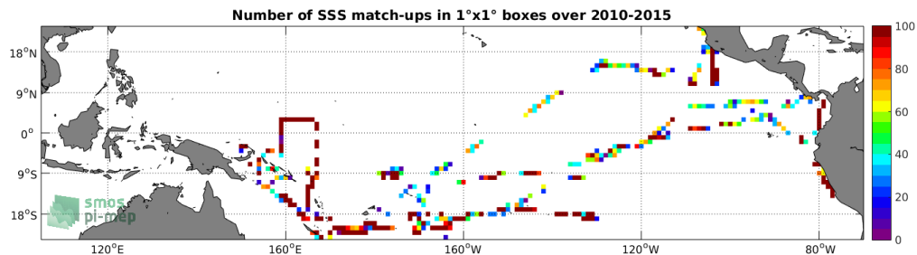
Figure 4: Number of SSS match-ups between TSG-GOSUD-Research-vessel SSS and the SMOS-L3-CATDS-CECOS-IFREMER-V2-1DAY-0.5DEG SSS product for the Tropical Pacific Ocean Pi-MEP region over 1^\circ \times 1^\circ boxes and for the full satellite product period.
