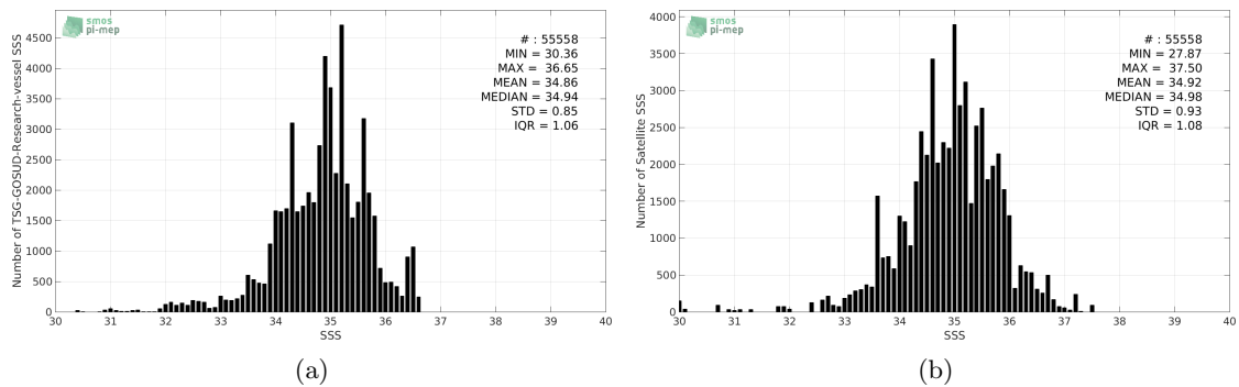
Figure 2: Histograms of SSS from TSG-GOSUD-Research-vessel (a) and SMOS-L3-CATDS-CECOS-IFREMER-V2-1DAY-0.5DEG (b) considering all match-up pairs per bins of 0.1 over the Tropical Pacific Ocean Pi-MEP region and for the full satellite product period.
