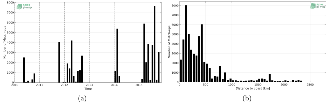
Figure 1: Number of match-ups between TSG-GOSUD-Research-vessel and SMOS-L3-CATDS-CECOS-IFREMER-V2-1DAY-0.5DEG SSS as a function of time (a) and as function of the distance to coast (b) over the Tropical Pacific Ocean Pi-MEP region and for the full satellite product period.
