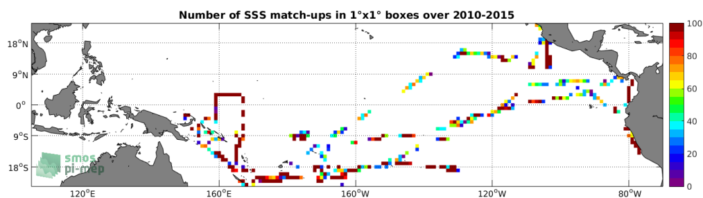
Figure 4: Number of SSS match-ups between TSG-GOSUD-Research-vessel SSS and the SMOS-L3-CATDS-CECOS-IFREMER-V2-1DAY-0.5DEG SSS product for the Tropical Pacific Ocean Pi-MEP region over 1^\circ \times 1^\circ boxes and for the full satellite product period.
