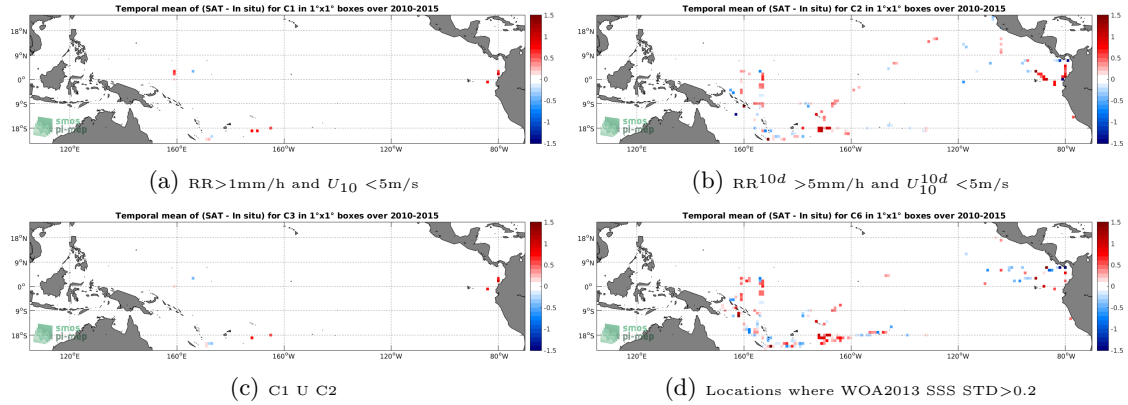
Figure 12: Temporal mean gridded over spatial boxes of size 1^\circ \times 1^\circ of \Delta SSS (SMOS-L3-CATDS-CECOS-IFREMER-V2-1DAY-0.5DEG - TSG-GOSUD-Research-vessel) for 4 different subdatasets corresponding to: RR > 1\text{mm/h} and U_{10} < 5\text{m/s} (a), RR^{10d} > 5\text{mm/h} and U_{10}^{10d} < 5\text{m/s} (b), C1 U C2 (c), Locations where WOA2013 SSS STD > 0.2 (d).
