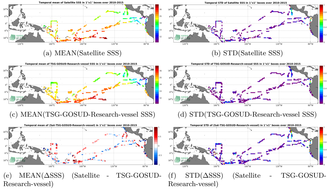
Figure 6: Temporal mean (left) and STD (right) of SSS from SMOS-L3-CATDS-CECOS-IFREMER-V2-1DAY-0.5DEG (top), TSG-GOSUD-Research-vessel (middle), and of \Delta SSS (Satellite - TSG-GOSUD-Research-vessel). Only match-up pairs are used to generate these maps.
