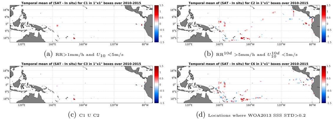
Figure 12: Temporal mean gridded over spatial boxes of size 1^\circ \times 1^\circ of \Delta SSS (SMOS-L3-CATDS-CECOS-IFREMER-V2-1DAY-0.5DEG - TSG-GOSUD-Research-vessel) for 4 different subdatasets corresponding to: RR > 1\text{mm/h} and U_{10} < 5\text{m/s} (a), RR^{10d} > 5\text{mm/h} and U_{10}^{10d} < 5\text{m/s} (b), C1 U C2 (c), Locations where WOA2013 SSS STD > 0.2 (d).
