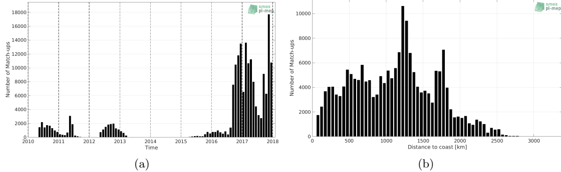
Figure 1: Number of match-ups between Surface drifters and SMOS SSS L3 v2 - Daily - 0.5 Deg (CATDS-CECOS-IFREMER) SSS as a function of time (a) and as function of the distance to coast (b) over the Tropical Pacific Ocean Pi-MEP region and for the full satellite product period.
