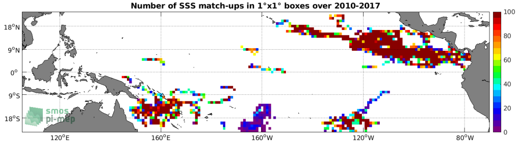
Figure 3: Number of SSS match-ups between Surface drifters SSS and the SMOS SSS L3 v2 - Daily - 0.5 Deg (CATDS-CECOS-IFREMER) SSS product for the Tropical Pacific Ocean Pi-MEP region over 1^\circ \times 1^\circ boxes and for the full satellite product period.
