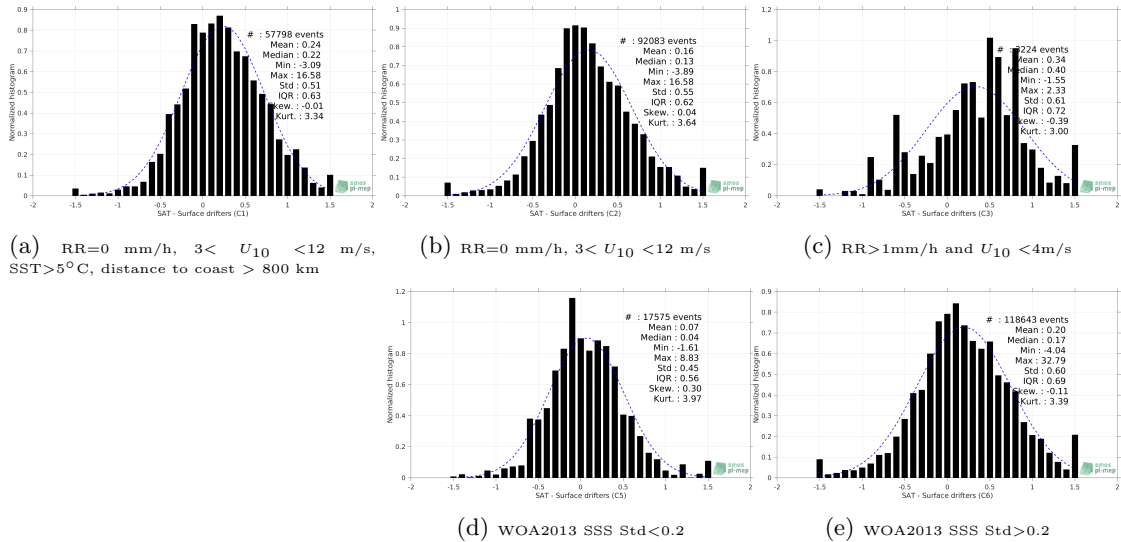
Figure 12: Normalized histogram of \Delta SSS (SMOS-L3-CATDS-CECOS-IFREMER-V2-1DAY-0.5DEG - Surface drifters) for 5 different subdatasets corresponding to: RR=0 mm/h, 3 < U_{10} < 12 m/s, SST >5^\circ\text{C} , distance to coast > 800 km (a), RR=0 mm/h, 3 < U_{10} < 12 m/s (b), RR >1 mm/h and U_{10} < 4 m/s (c), WOA2013 SSS Std <0.2 (d), WOA2013 SSS Std >0.2 (e).
