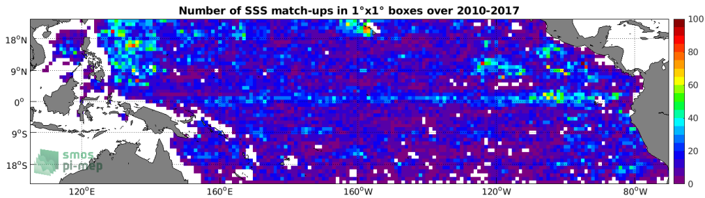
Figure 4: Number of SSS match-ups between Argo SSS and the SMOS SSS L3 v2 - Daily - 0.5 Deg (CATDS-CECOS-IFREMER) SSS product for the Tropical Pacific Ocean Pi-MEP region over 1°x1° boxes and for the full satellite product period.
