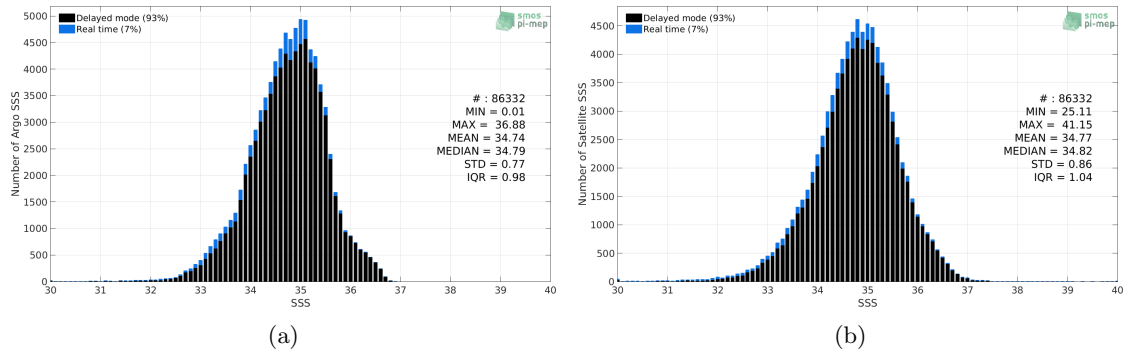
Figure 2: Histograms of SSS from Argo (a) and SMOS SSS L3 v2 - Daily - 0.5 Deg (CATDS-CECOS-IFREMER) (b) considering all match-up pairs per bins of 0.1 over the Tropical Pacific Ocean Pi-MEP region and for the full satellite product period.
