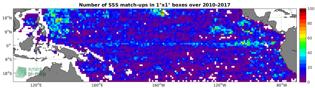
Figure 4: Number of SSS match-ups between Argo SSS and the SMOS SSS L3 v2 - Daily - 0.5 Deg (CATDS-CECOS-IFREMER) SSS product for the Tropical Pacific Ocean Pi-MEP region over 1^\circ \times 1^\circ boxes and for the full satellite product period.
