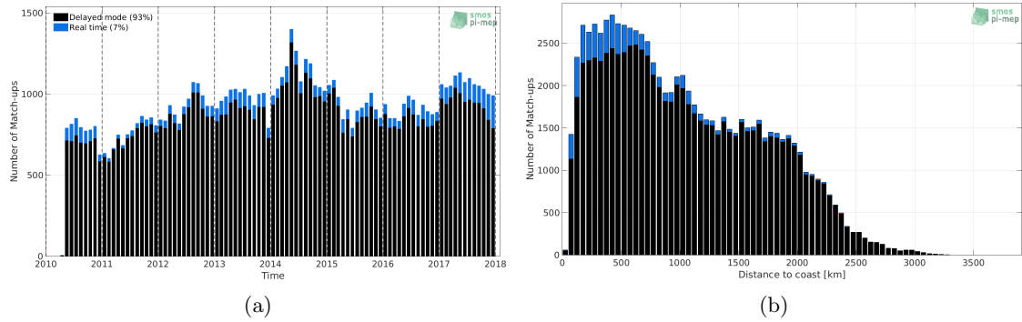
Figure 1: Number of match-ups between Argo and SMOS SSS L3 v2 - Daily - 0.5 Deg (CATDS-CECOS-IFREMER) SSS as a function of time (a) and as function of the distance to coast (b) over the Tropical Pacific Ocean Pi-MEP region and for the full satellite product period.
