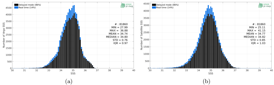
Figure 2: Histograms of SSS from Argo (a) and SMOS L3 v2 - Daily - 0.5 Deg (CATDS-CECOS-IFREMER) (b) considering all match-up pairs per bins of 0.1 over the Tropical Pacific Ocean Pi-MEP region and for the full satellite product period.
