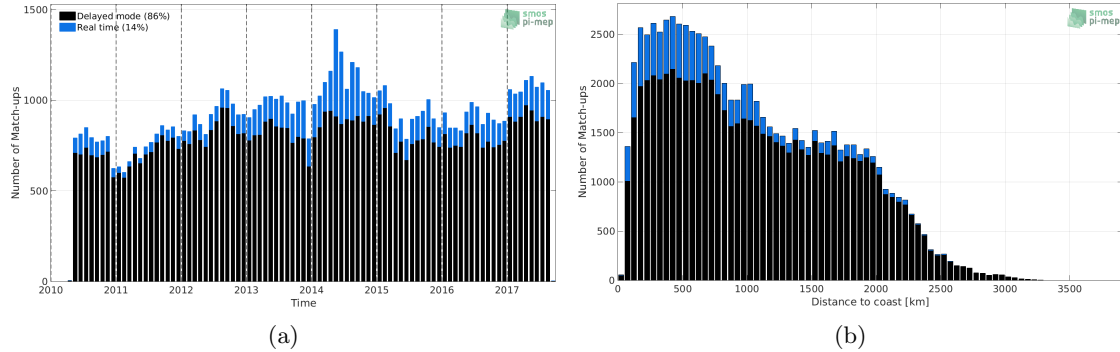
Figure 1: Number of match-ups between Argo and SMOS L3 v2 - Daily - 0.5 Deg (CATDS-CECOS-IFREMER) SSS as a function of time (a) and as function of the distance to coast (b) over the Tropical Pacific Ocean Pi-MEP region and for the full satellite product period.
