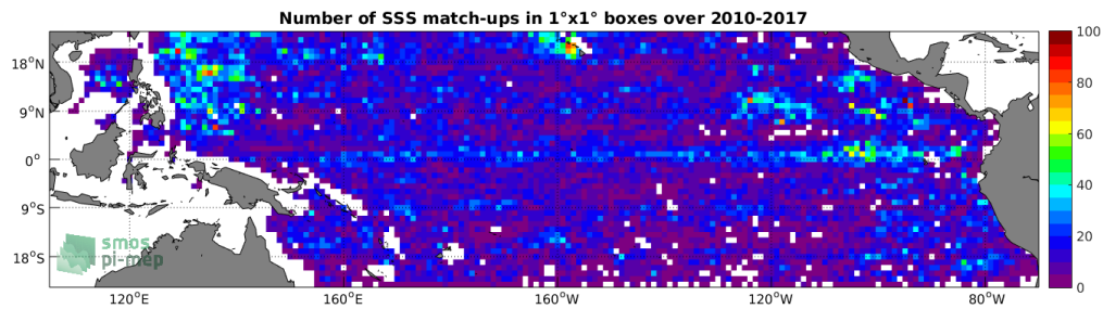
Figure 4: Number of SSS match-ups between Argo SSS and the SMOS L3 v2 - Daily - 0.5 Deg (CATDS-CECOS-IFREMER) SSS product for the Tropical Pacific Ocean Pi-MEP region over 1^\circ \times 1^\circ boxes and for the full satellite product period.
