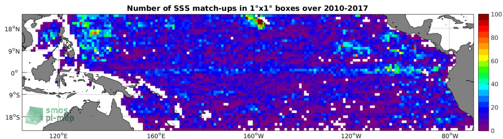
Figure 4: Number of SSS match-ups between Argo SSS and the SMOS-L3-CATDS-CECOS-IFREMER-V2-1DAY-0.5DEG SSS product for the Tropical Pacific Ocean Pi-MEP region over 1^\circ \times 1^\circ boxes and for the full satellite product period.
