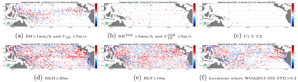
Figure 12: Temporal mean gridded over spatial boxes of size 1°x1° of \Delta SSS (SMOS-L3-CATDS-CECOS-IFREMER-V2-1DAY-0.5DEG - Argo) for 6 different subdatasets corresponding to:RR>1mm/h and U_{10} < 5m/s (a), RR^{10d} > 5mm/h and U_{10}^{10d} < 5m/s (b), C1 U C2 (c),MLD<20m (d),BLT>10m (e),Locations where WOA2013 SSS STD>0.2 (f).
