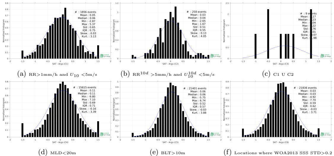
Figure 13: Normalized histogram of \Delta SSS (SMOS-L3-CATDS-CECOS-IFREMER-V2-1DAY-0.5DEG - Argo) for 6 different subdatasets corresponding to: RR>1mm/h and U_{10} < 5m/s (a), RR^{10d} > 5mm/h and U_{10}^{10d} < 5m/s (b), C1 U C2 (c),MLD<20m (d),BLT>10m (e),Locations where WOA2013 SSS STD>0.2 (f).
