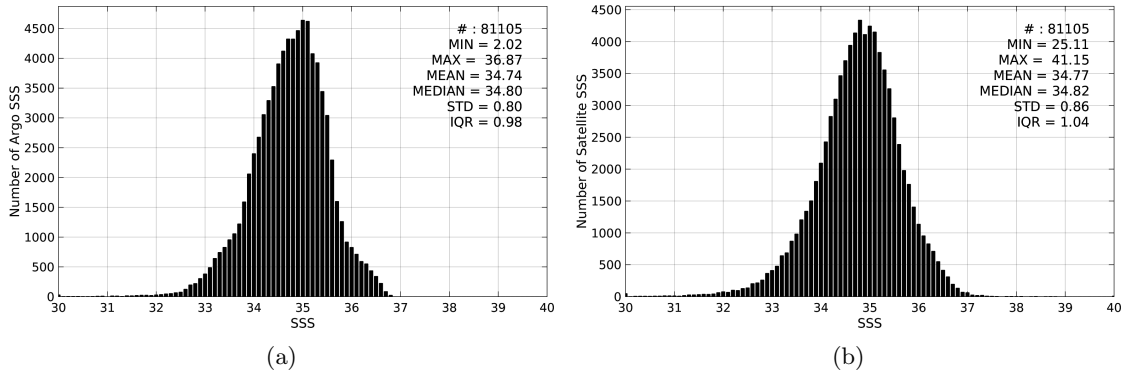
Figure 2: Histograms of SSS from Argo (a) and SMOS-L3-CATDS-CECOS-IFREMER-V2-1DAY-0.5DEG (b) considering all match-up pairs per bins of 0.1 over the Tropical Pacific Ocean Pi-MEP region and for the full satellite product period.
