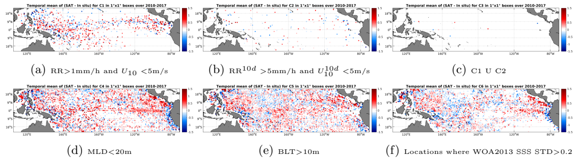
Figure 12: Temporal mean gridded over spatial boxes of size 1^\circ \times 1^\circ of \Delta SSS (SMOS-L3-CATDS-CECOS-IFREMER-V2-1DAY-0.5DEG - Argo) for 6 different subdatasets corresponding to: RR>1mm/h and U_{10} < 5\text{m/s} (a), RR^{10d} > 5\text{mm/h} and U_{10}^{10d} < 5\text{m/s} (b), C1 U C2 (c),MLD<20m (d),BLT>10m (e),Locations where WOA2013 SSS STD>0.2 (f).
