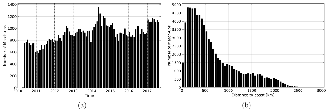
Figure 1: Number of match-ups between Argo and SMOS-L3-CATDS-CECOS-IFREMER-V2-1DAY-0.5DEG SSS as a function of time (a) and as function of the distance to coast (b) over the Tropical Pacific Ocean Pi-MEP region and for the full satellite product period.
