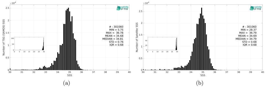
Figure 3: Histograms of SSS from TSG (SAMOS) (a) and SMOS SSS L3 v335 - Monthly - 25 km (CATDS-CPDC) (b) considering all match-up pairs per bins of 0.1 over the Tropical Pacific Ocean Pi-MEP region and for the full satellite product period.
