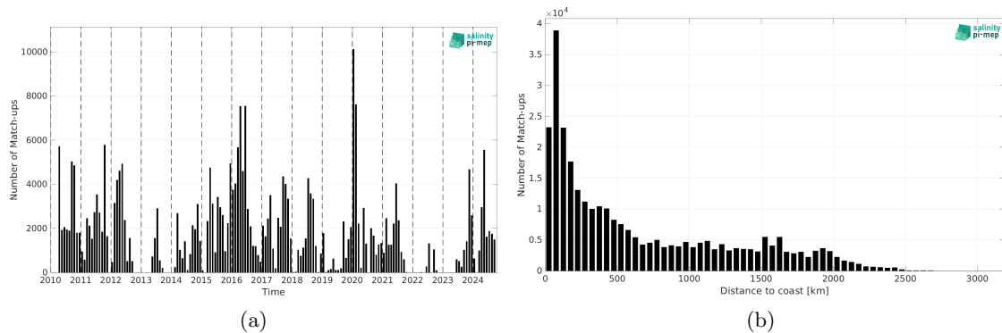
Figure 2: Number of match-ups between TSG (SAMOS) and SMOS SSS L3 v335 - Monthly - 25 km (CATDS-CPDC) SSS as a function of time (a) and as function of the distance to coast (b) over the Tropical Pacific Ocean Pi-MEP region and for the full satellite product period.
