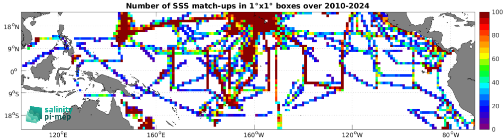
Figure 5: Number of SSS match-ups between TSG (SAMOS) SSS and the SMOS SSS L3 v335 - Monthly - 25 km (CATDS-CPDC) SSS product for the Tropical Pacific Ocean Pi-MEP region over 1^\circ \times 1^\circ boxes and for the full satellite product period.
