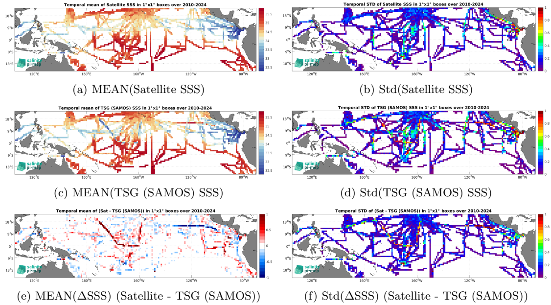
Figure 7: Temporal mean (left) and Std (right) of SSS from SMOS SSS L3 v335 - Monthly - 25 km (CATDS-CPDC) (top), TSG (SAMOS) (middle), and of \Delta SSS (Satellite - TSG (SAMOS)). Only match-up pairs are used to generate these maps.
