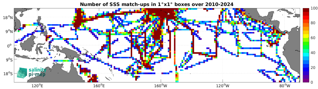
Figure 5: Number of SSS match-ups between TSG (SAMOS) SSS and the SMOS SSS L3 v335 - Monthly - 25 km (CATDS-CPDC) SSS product for the Tropical Pacific Ocean Pi-MEP region over 1^\circ \times 1^\circ boxes and for the full satellite product period.
