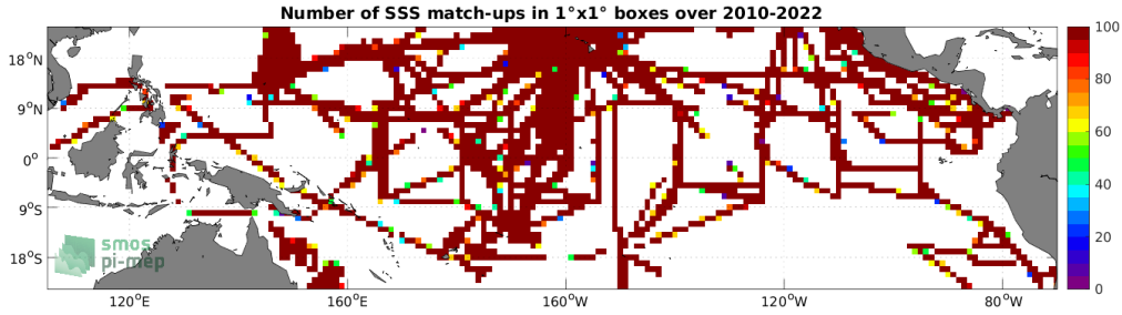
Figure 4: Number of SSS match-ups between TSG (SAMOS) SSS and the SMOS SSS L3 v335 - Monthly - 25 km (CATDS-CPDC) SSS product for the Tropical Pacific Ocean Pi-MEP region over 1^\circ \times 1^\circ boxes and for the full satellite product period.
