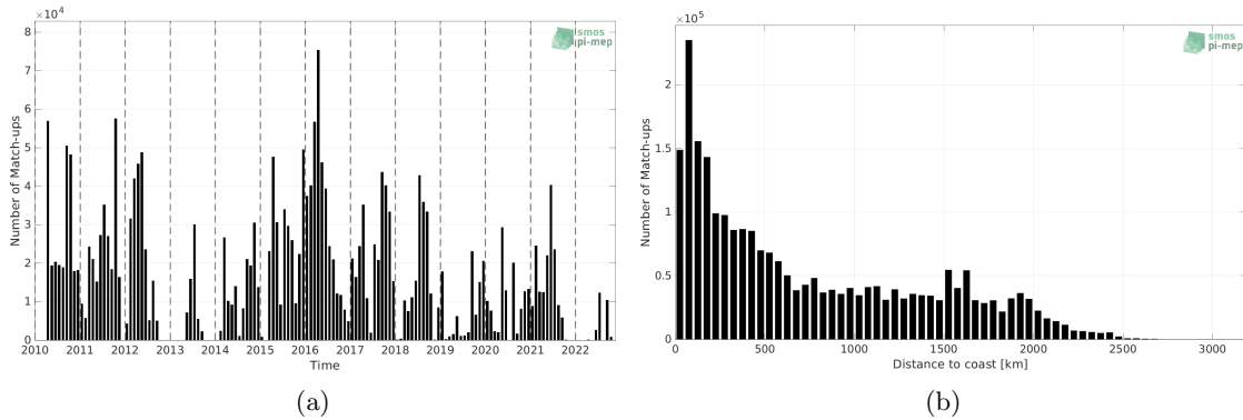
Figure 1: Number of match-ups between TSG (SAMOS) and SMOS SSS L3 v335 - Monthly - 25 km (CATDS-CPDC) SSS as a function of time (a) and as function of the distance to coast (b) over the Tropical Pacific Ocean Pi-MEP region and for the full satellite product period.
