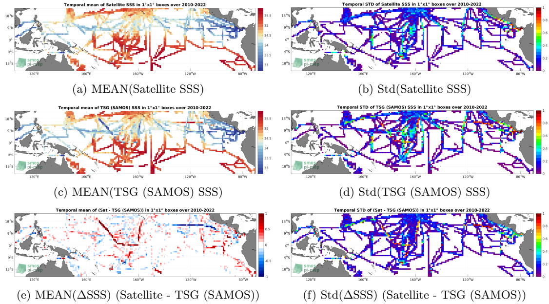
Figure 6: Temporal mean (left) and Std (right) of SSS from SMOS SSS L3 v335 - Monthly - 25 km (CATDS-CPDC) (top), TSG (SAMOS) (middle), and of \Delta SSS (Satellite - TSG (SAMOS)). Only match-up pairs are used to generate these maps.
