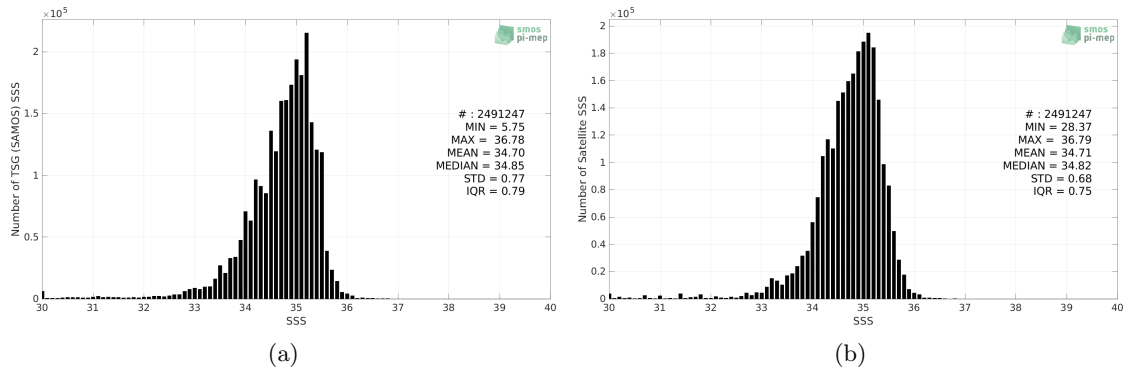
Figure 2: Histograms of SSS from TSG (SAMOS) (a) and SMOS SSS L3 v335 - Monthly - 25 km (CATDS-CPDC) (b) considering all match-up pairs per bins of 0.1 over the Tropical Pacific Ocean Pi-MEP region and for the full satellite product period.
