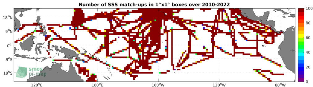
Figure 4: Number of SSS match-ups between TSG (SAMOS) SSS and the SMOS SSS L3 v335 - Monthly - 25 km (CATDS-CPDC) SSS product for the Tropical Pacific Ocean Pi-MEP region over 1^\circ \times 1^\circ boxes and for the full satellite product period.
