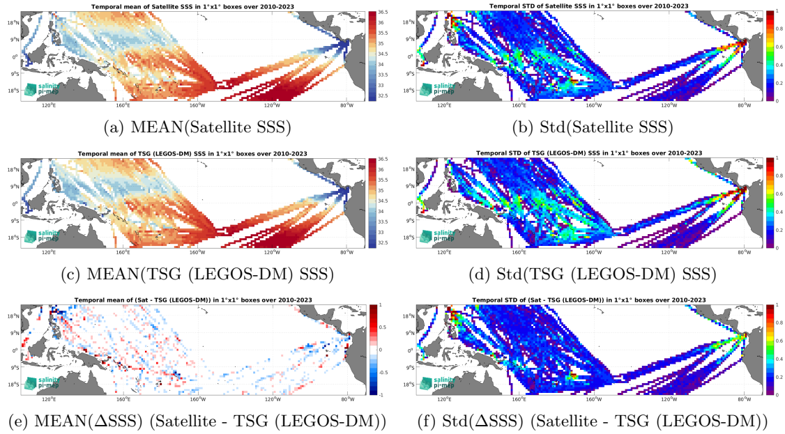
Figure 7: Temporal mean (left) and Std (right) of SSS from SMOS SSS L3 v335 - Monthly - 25 km (CATDS-CPDC) (top), TSG (LEGOS-DM) (middle), and of \Delta SSS (Satellite - TSG (LEGOS-DM)). Only match-up pairs are used to generate these maps.
