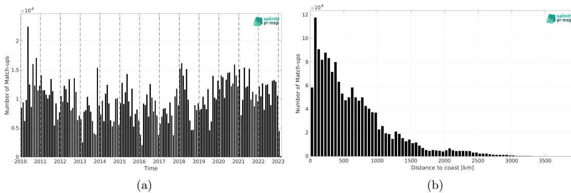
Figure 2: Number of match-ups between TSG (LEGOS-DM) and SMOS SSS L3 v335 - Monthly - 25 km (CATDS-CPDC) SSS as a function of time (a) and as function of the distance to coast (b) over the Tropical Pacific Ocean Pi-MEP region and for the full satellite product period.
