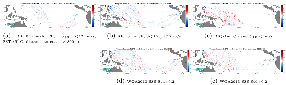
Figure 14: Temporal mean gridded over spatial boxes of size 1^\circ \times 1^\circ of \Delta SSS (SMOS SSS L3 v335 - Monthly - 25 km (CATDS-CPDC) - TSG (LEGOS-DM)) for 5 different subdatasets corresponding to: RR=0 mm/h, 3 < U_{10} < 12 m/s, SST > 5^\circ\text{C} , distance to coast > 800 km (a), RR=0 mm/h, 3 < U_{10} < 12 m/s (b), RR > 1 mm/h and U_{10} < 4 m/s (c), WOA2013 SSS Std < 0.2 (d), WOA2013 SSS Std > 0.2 (e).
