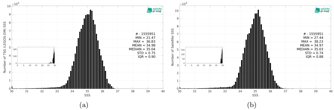
Figure 3: Histograms of SSS from TSG (LEGOS-DM) (a) and SMOS SSS L3 v335 - Monthly - 25 km (CATDS-CPDC) (b) considering all match-up pairs per bins of 0.1 over the Tropical Pacific Ocean Pi-MEP region and for the full satellite product period.
