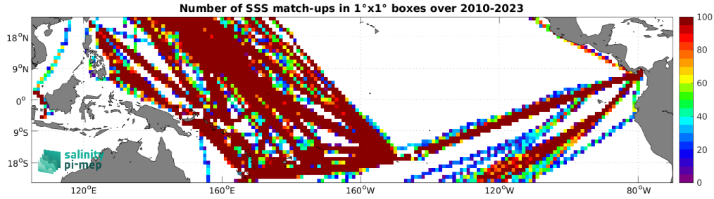
Figure 5: Number of SSS match-ups between TSG (LEGOS-DM) SSS and the SMOS SSS L3 v335 - Monthly - 25 km (CATDS-CPDC) SSS product for the Tropical Pacific Ocean Pi-MEP region over 1^\circ \times 1^\circ boxes and for the full satellite product period.
