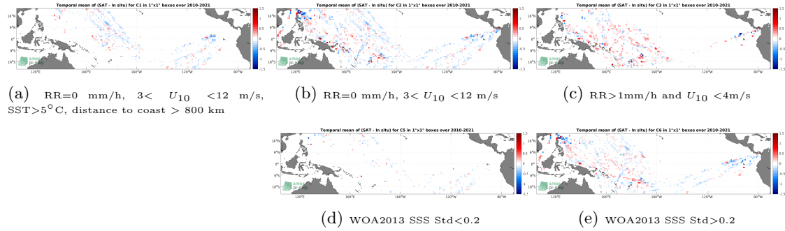
Figure 12: Temporal mean gridded over spatial boxes of size 1^{\circ}\times 1^{\circ} of \Delta\text{SSS} (SMOS SSS L3 v335 - Monthly - 25 km (CATDS-CPDC) - TSG (LEGOS-DM)) for 5 different subdatasets corresponding to:RR=0 mm/h, 3 < U_{10} < 12 m/s, SST >5^{\circ}\text{C} , distance to coast > 800 km (a), RR=0 mm/h, 3 < U_{10} < 12 m/s (b), RR >1 mm/h and U_{10} < 4 m/s (c), WOA2013 SSS Std <0.2 (d), WOA2013 SSS Std >0.2 (e).
