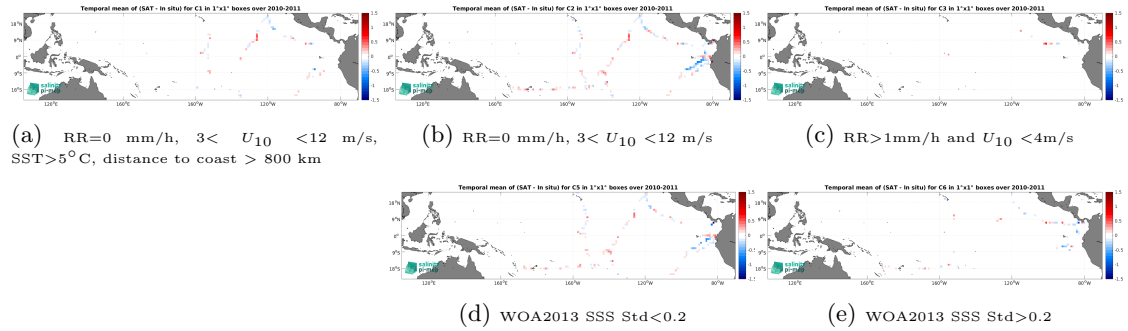
Figure 12: Temporal mean gridded over spatial boxes of size 1^{\circ}\times 1^{\circ} of \Delta SSS (SMOS SSS L3 v335 - Monthly - 25 km (CATDS-CPDC) - TSG (GOSUD-Sailing-ship)) for 5 different subdatasets corresponding to:RR=0 mm/h, 3 < U_{10} < 12 m/s, SST >5^{\circ}\text{C} , distance to coast > 800 km (a), RR=0 mm/h, 3 < U_{10} < 12 m/s (b), RR >1 mm/h and U_{10} < 4 m/s (c), WOA2013 SSS Std <0.2 (d), WOA2013 SSS Std >0.2 (e).
