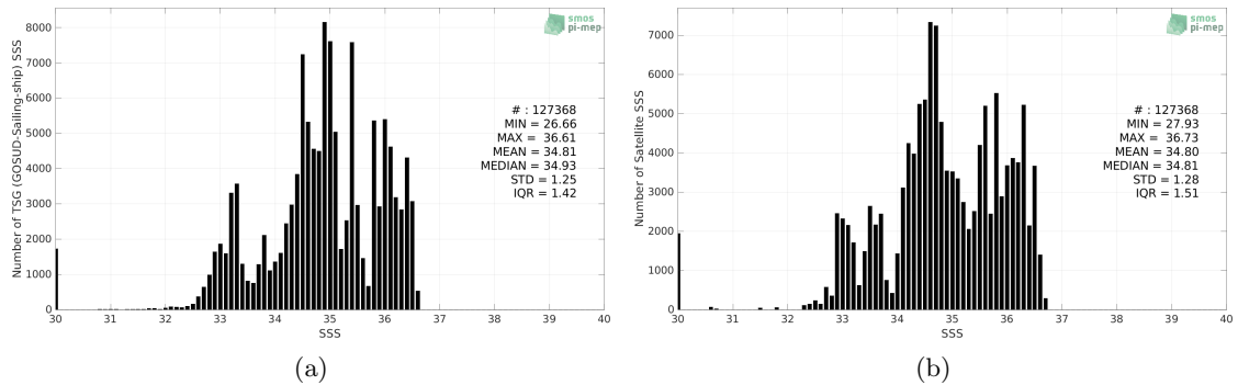
Figure 2: Histograms of SSS from TSG (GOSUD-Sailing-ship) (a) and SMOS SSS L3 v335 - Monthly - 25 km (CATDS-CPDC) (b) considering all match-up pairs per bins of 0.1 over the Tropical Pacific Ocean Pi-MEP region and for the full satellite product period.
