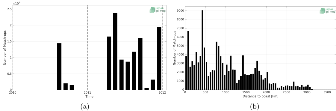
Figure 1: Number of match-ups between TSG (GOSUD-Sailing-ship) and SMOS SSS L3 v335 - Monthly - 25 km (CATDS-CPDC) SSS as a function of time (a) and as function of the distance to coast (b) over the Tropical Pacific Ocean Pi-MEP region and for the full satellite product period.
