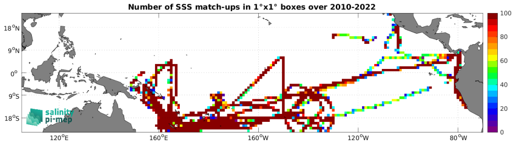
Figure 5: Number of SSS match-ups between TSG (GOSUD-Research-vessel) SSS and the SMOS SSS L3 v335 - Monthly - 25 km (CATDS-CPDC) SSS product for the Tropical Pacific Ocean Pi-MEP region over 1^\circ \times 1^\circ boxes and for the full satellite product period.
