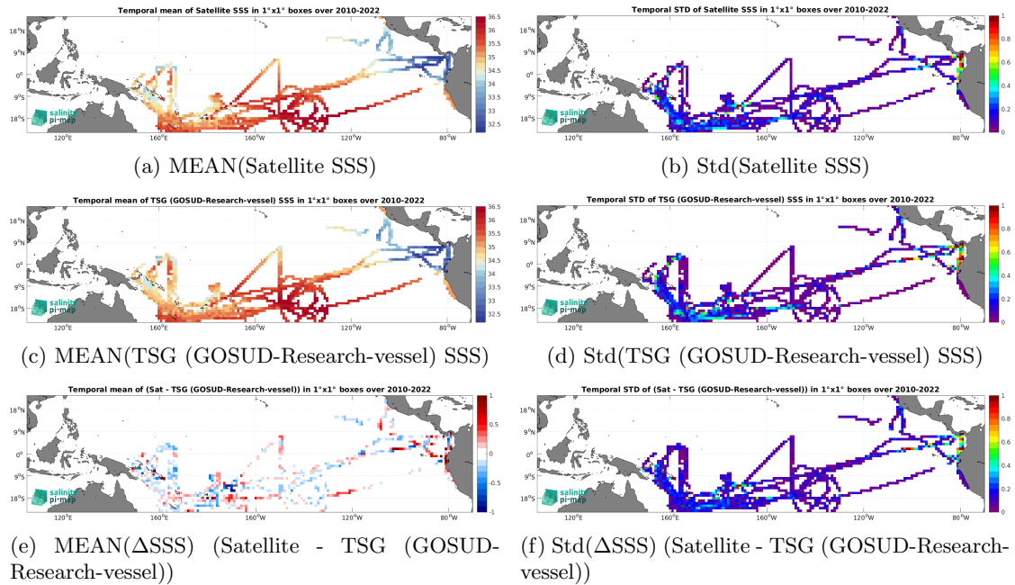
Figure 7: Temporal mean (left) and Std (right) of SSS from SMOS SSS L3 v335 - Monthly - 25 km (CATDS-CPDC) (top), TSG (GOSUD-Research-vessel) (middle), and of \Delta SSS (Satellite - TSG (GOSUD-Research-vessel)). Only match-up pairs are used to generate these maps.
