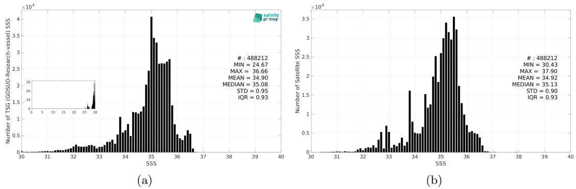
Figure 3: Histograms of SSS from TSG (GOSUD-Research-vessel) (a) and SMOS SSS L3 v335 - Monthly - 25 km (CATDS-CPDC) (b) considering all match-up pairs per bins of 0.1 over the Tropical Pacific Ocean Pi-MEP region and for the full satellite product period.
