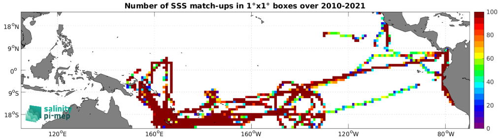
Figure 5: Number of SSS match-ups between TSG (GOSUD-Research-vessel) SSS and the SMOS SSS L3 v335 - Monthly - 25 km (CATDS-CPDC) SSS product for the Tropical Pacific Ocean Pi-MEP region over 1^\circ \times 1^\circ boxes and for the full satellite product period.
