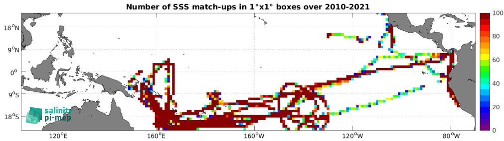
Figure 4: Number of SSS match-ups between TSG (GOSUD-Research-vessel) SSS and the SMOS SSS L3 v335 - Monthly - 25 km (CATDS-CPDC) SSS product for the Tropical Pacific Ocean Pi-MEP region over 1^\circ \times 1^\circ boxes and for the full satellite product period.
