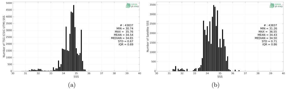
Figure 2: Histograms of SSS from TSG (CSIC-UTM) (a) and SMOS SSS L3 v335 - Monthly - 25 km (CATDS-CPDC) (b) considering all match-up pairs per bins of 0.1 over the Tropical Pacific Ocean Pi-MEP region and for the full satellite product period.
