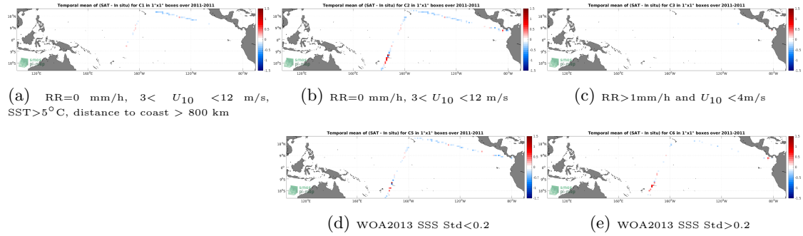
Figure 12: Temporal mean gridded over spatial boxes of size 1^{\circ}\times 1^{\circ} of \Delta\text{SSS} (SMOS SSS L3 v335 - Monthly - 25 km (CATDS-CPDC) - TSG (CSIC-UTM)) for 5 different subdatasets corresponding to:RR=0 mm/h, 3 < U_{10} < 12 m/s, SST >5^{\circ}\text{C} , distance to coast > 800 km (a), RR=0 mm/h, 3 < U_{10} < 12 m/s (b), RR >1 mm/h and U_{10} < 4 m/s (c), WOA2013 SSS Std <0.2 (d), WOA2013 SSS Std >0.2 (e).
