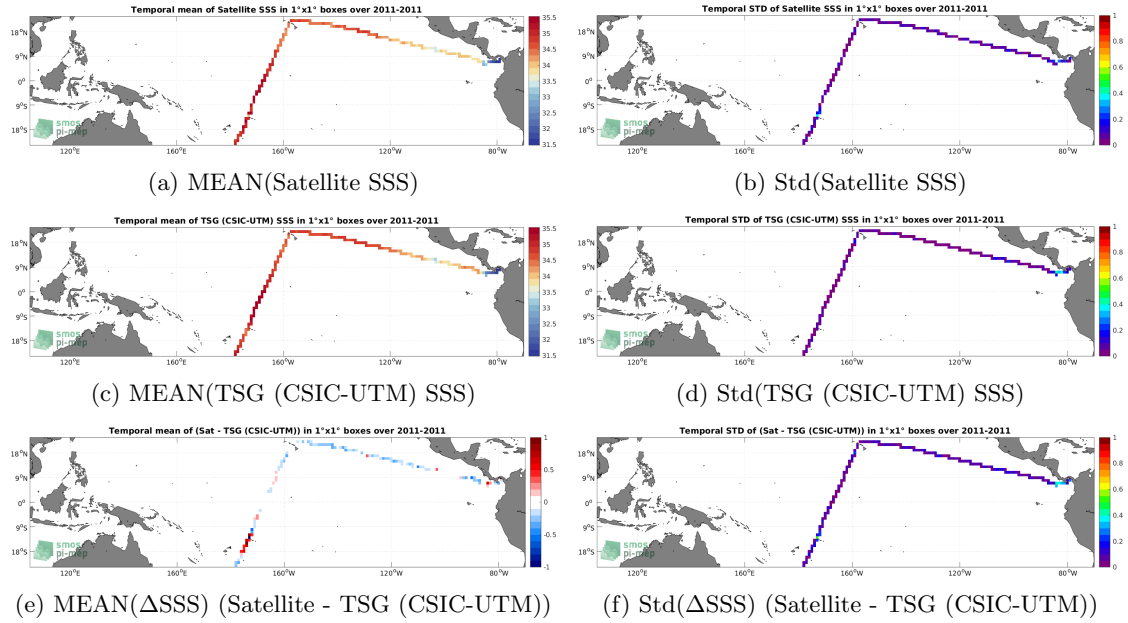
Figure 6: Temporal mean (left) and Std (right) of SSS from SMOS SSS L3 v335 - Monthly - 25 km (CATDS-CPDC) (top), TSG (CSIC-UTM) (middle), and of \Delta SSS (Satellite - TSG (CSIC-UTM)). Only match-up pairs are used to generate these maps.
