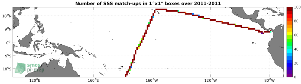
Figure 4: Number of SSS match-ups between TSG (CSIC-UTM) SSS and the SMOS SSS L3 v335 - Monthly - 25 km (CATDS-CPDC) SSS product for the Tropical Pacific Ocean Pi-MEP region over 1^\circ \times 1^\circ boxes and for the full satellite product period.
