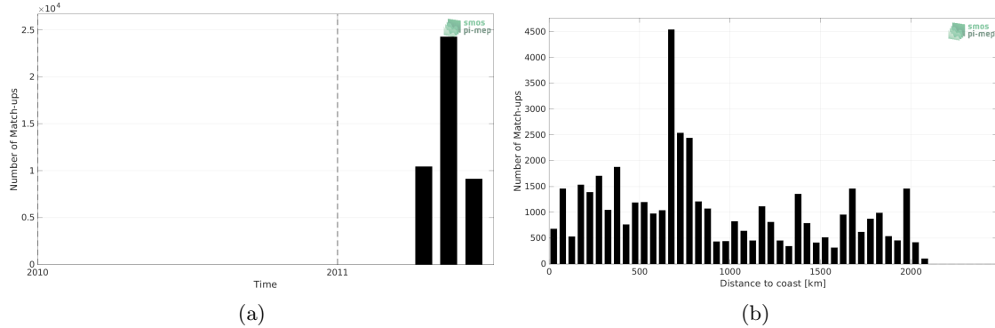
Figure 1: Number of match-ups between TSG (CSIC-UTM) and SMOS SSS L3 v335 - Monthly - 25 km (CATDS-CPDC) SSS as a function of time (a) and as function of the distance to coast (b) over the Tropical Pacific Ocean Pi-MEP region and for the full satellite product period.
