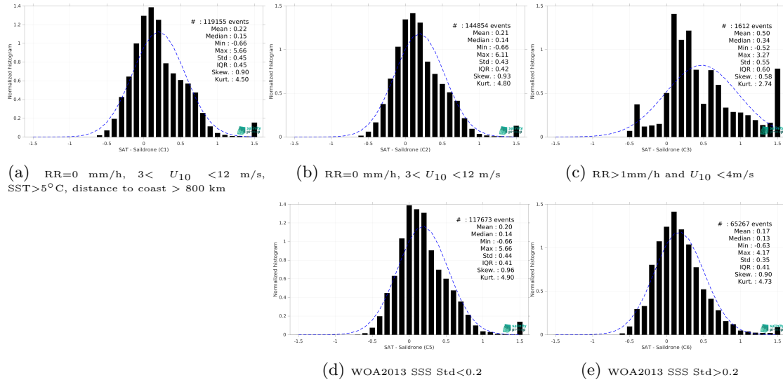
Figure 15: Normalized histogram of \Delta SSS (SMOS SSS L3 v335 - Monthly - 25 km (CATDS-CPDC) - Ssaldrone) for 5 different subdatasets corresponding to: RR=0 mm/h, 3 < U_{10} < 12 m/s, SST > 5°C, distance to coast > 800 km (a), RR=0 mm/h, 3 < U_{10} < 12 m/s (b), RR > 1mm/h and U_{10} < 4 m/s (c), WOA2013 SSS Std < 0.2 (d), WOA2013 SSS Std > 0.2 (e).
