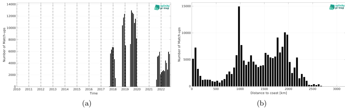
Figure 2: Number of match-ups between Saildrone and SMOS SSS L3 v335 - Monthly - 25 km (CATDS-CPDC) SSS as a function of time (a) and as function of the distance to coast (b) over the Tropical Pacific Ocean Pi-MEP region and for the full satellite product period.
