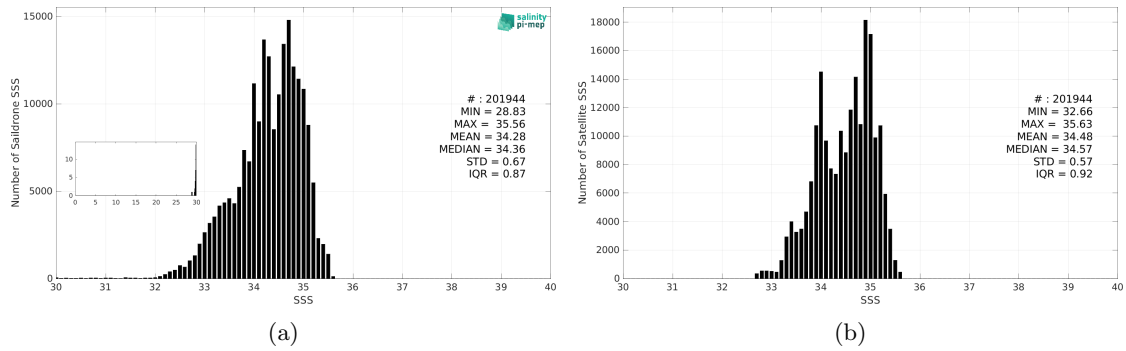
Figure 3: Histograms of SSS from Saildrone (a) and SMOS SSS L3 v335 - Monthly - 25 km (CATDS-CPDC) (b) considering all match-up pairs per bins of 0.1 over the Tropical Pacific Ocean Pi-MEP region and for the full satellite product period.
