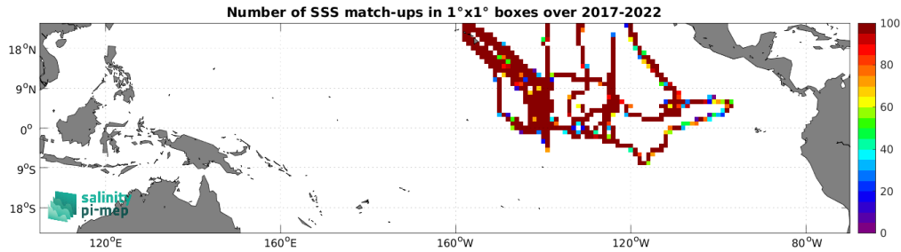
Figure 4: Number of SSS match-ups between Saildrone SSS and the SMOS SSS L3 v335 - Monthly - 25 km (CATDS-CPDC) SSS product for the Tropical Pacific Ocean Pi-MEP region over 1^\circ \times 1^\circ boxes and for the full satellite product period.
