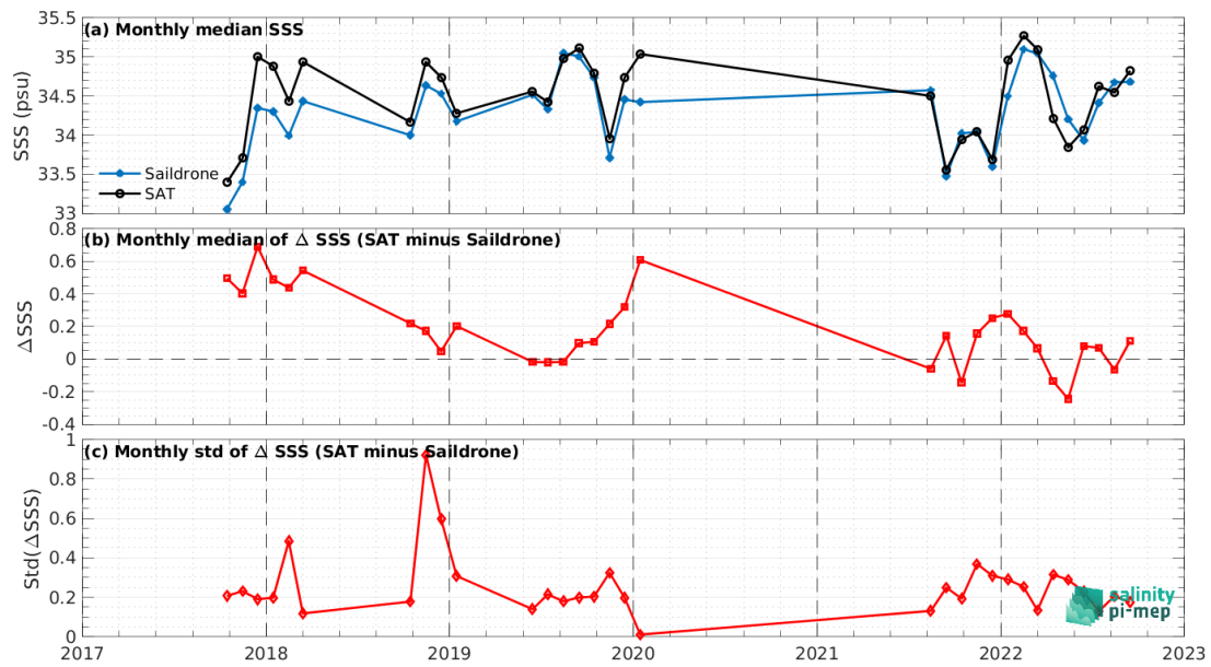
Figure 7: Time series of the monthly median SSS (top), median of \Delta SSS (Satellite - Sairdron) and Std of \Delta SSS (Satellite - Sairdron) over the Tropical Pacific Ocean Pi-MEP region considering all match-ups collected by the Pi-MEP.
