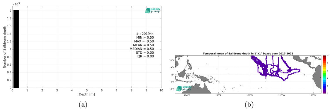
Figure 3: Histograms of the depth of the upper level SSS measurements from Saldrone in the Match-up DataBase for the Tropical Pacific Ocean Pi-MEP region (a) and temporal mean spatial distribution of pressure of the in situ SSS data over 1^\circ \times 1^\circ boxes and for the full satellite product period (b).
