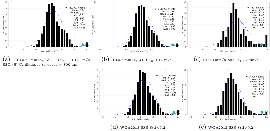
Figure 13: Normalized histogram of \Delta SSS (SMOS SSS L3 v335 - Monthly - 25 km (CATDS-CPDC) - Ssaldrone) for 5 different subdatasets corresponding to: RR=0 mm/h, 3 < U_{10} < 12 m/s, SST>5°C, distance to coast > 800 km (a), RR=0 mm/h, 3 < U_{10} < 12 m/s (b), RR>1mm/h and U_{10} < 4 m/s (c), WOA2013 SSS Std<0.2 (d), WOA2013 SSS Std>0.2 (e).
