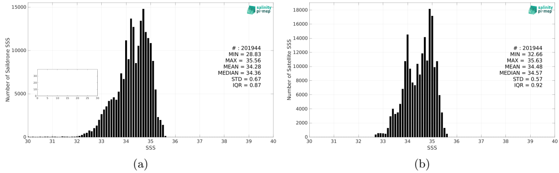
Figure 2: Histograms of SSS from Saldrone (a) and SMOS SSS L3 v335 - Monthly - 25 km (CATDS-CPDC) (b) considering all match-up pairs per bins of 0.1 over the Tropical Pacific Ocean Pi-MEP region and for the full satellite product period.
