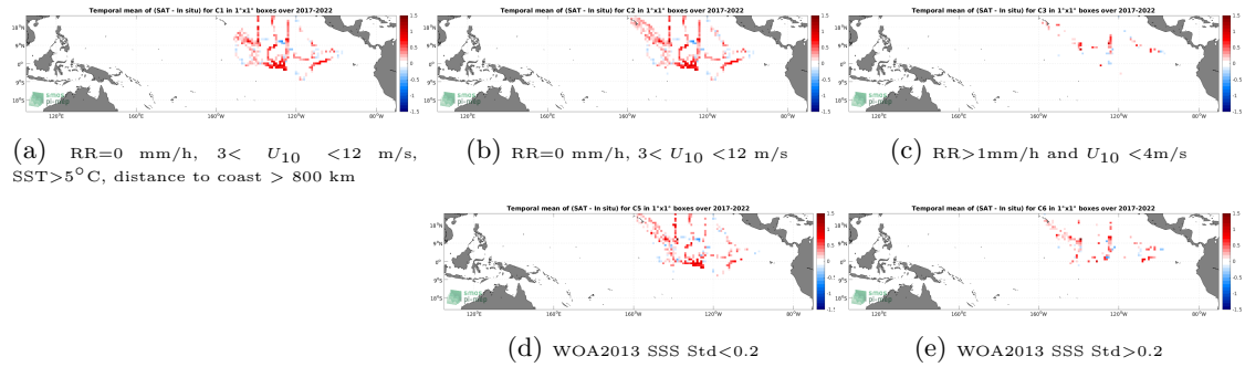
Figure 12: Temporal mean gridded over spatial boxes of size 1^\circ \times 1^\circ of \Delta SSS (SMOS SSS L3 v335 - Monthly - 25 km (CATDS-CPDC) - Saildrone) for 5 different subdatasets corresponding to: RR=0 mm/h, 3 < U_{10} < 12 m/s, SST > 5^\circ\text{C} , distance to coast > 800 km (a), RR=0 mm/h, 3 < U_{10} < 12 m/s (b), RR > 1 mm/h and U_{10} < 4 m/s (c), WOA2013 SSS Std < 0.2 (d), WOA2013 SSS Std > 0.2 (e).
