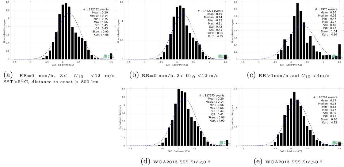
Figure 13: Normalized histogram of \Delta SSS (SMOS SSS L3 v335 - Monthly - 25 km (CATDS-CPDC) - Salldrone) for 5 different subdatasets corresponding to: RR=0 mm/h, 3 < U_{10} < 12 m/s, SST>5°C, distance to coast > 800 km (a), RR=0 mm/h, 3 < U_{10} < 12 m/s (b), RR>1mm/h and U_{10} < 4 m/s (c), WOA2013 SSS Std<0.2 (d), WOA2013 SSS Std>0.2 (e).
