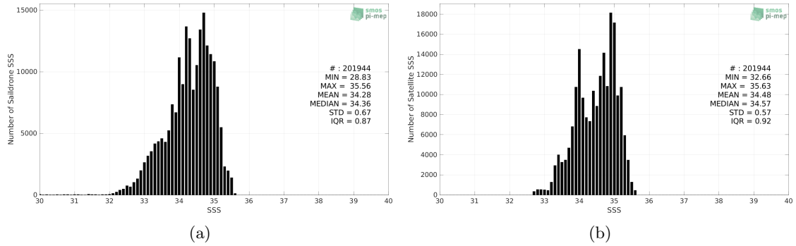
Figure 2: Histograms of SSS from Saildrone (a) and SMOS SSS L3 v335 - Monthly - 25 km (CATDS-CPDC) (b) considering all match-up pairs per bins of 0.1 over the Tropical Pacific Ocean Pi-MEP region and for the full satellite product period.
