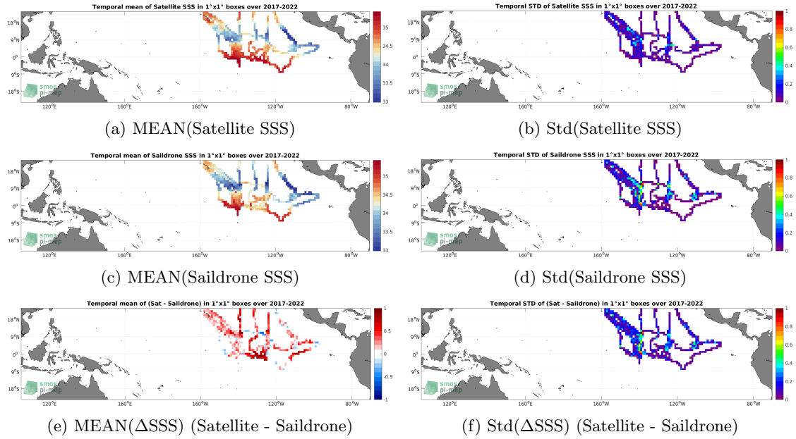
Figure 6: Temporal mean (left) and Std (right) of SSS from SMOS SSS L3 v335 - Monthly - 25 km (CATDS-CPDC) (top), Saildrone (middle), and of \Delta SSS (Satellite - Saildrone). Only match-up pairs are used to generate these maps.
