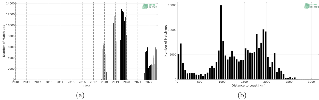
Figure 1: Number of match-ups between Saildrone and SMOS SSS L3 v335 - Monthly - 25 km (CATDS-CPDC) SSS as a function of time (a) and as function of the distance to coast (b) over the Tropical Pacific Ocean Pi-MEP region and for the full satellite product period.
