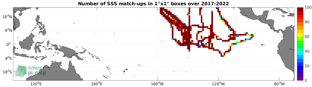
Figure 4: Number of SSS match-ups between Saildrone SSS and the SMOS SSS L3 v335 - Monthly - 25 km (CATDS-CPDC) SSS product for the Tropical Pacific Ocean Pi-MEP region over 1^\circ \times 1^\circ boxes and for the full satellite product period.
