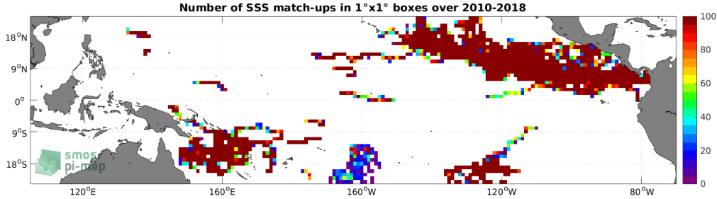
Figure 3: Number of SSS match-ups between Surface drifters SSS and the SMOS SSS L3 v335 - Monthly - 25 km (CATDS-CPDC) SSS product for the Tropical Pacific Ocean Pi-MEP region over 1^\circ \times 1^\circ boxes and for the full satellite product period.
