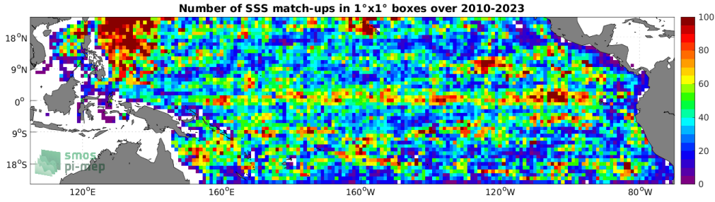
Figure 4: Number of SSS match-ups between Argo SSS and the SMOS SSS L3 v335 - Monthly - 25 km (CATDS-CPDC) SSS product for the Tropical Pacific Ocean Pi-MEP region over 1^\circ \times 1^\circ boxes and for the full satellite product period.
