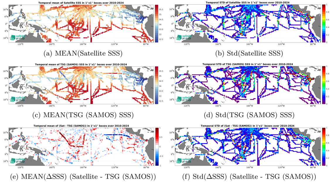
Figure 7: Temporal mean (left) and Std (right) of SSS from SMOS SSS L3 v335 - 10 Days - 25 km (CATDS-CPDC) (top), TSG (SAMOS) (middle), and of \Delta SSS (Satellite - TSG (SAMOS)). Only match-up pairs are used to generate these maps.
