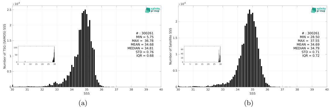
Figure 3: Histograms of SSS from TSG (SAMOS) (a) and SMOS SSS L3 v335 - 10 Days - 25 km (CATDS-CPDC) (b) considering all match-up pairs per bins of 0.1 over the Tropical Pacific Ocean Pi-MEP region and for the full satellite product period.
