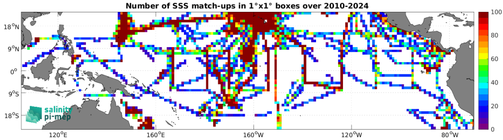
Figure 5: Number of SSS match-ups between TSG (SAMOS) SSS and the SMOS SSS L3 v335 - 10 Days - 25 km (CATDS-CPDC) SSS product for the Tropical Pacific Ocean Pi-MEP region over 1^\circ \times 1^\circ boxes and for the full satellite product period.
