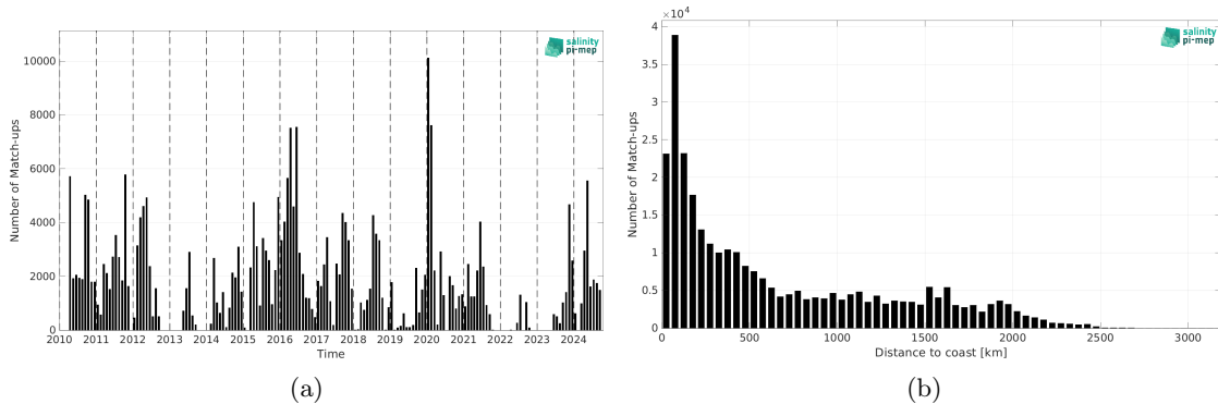
Figure 2: Number of match-ups between TSG (SAMOS) and SMOS SSS L3 v335 - 10 Days - 25 km (CATDS-CPDC) SSS as a function of time (a) and as function of the distance to coast (b) over the Tropical Pacific Ocean Pi-MEP region and for the full satellite product period.
