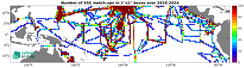
Figure 5: Number of SSS match-ups between TSG (SAMOS) SSS and the SMOS SSS L3 v335 - 10 Days - 25 km (CATDS-CPDC) SSS product for the Tropical Pacific Ocean Pi-MEP region over 1^\circ \times 1^\circ boxes and for the full satellite product period.
