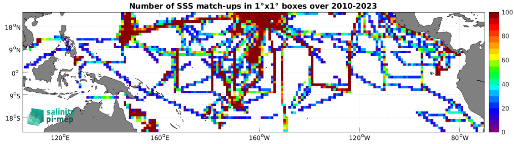
Figure 4: Number of SSS match-ups between TSG (SAMOS) SSS and the SMOS SSS L3 v335 - 10 Days - 25 km (CATDS-CPDC) SSS product for the Tropical Pacific Ocean Pi-MEP region over 1^\circ \times 1^\circ boxes and for the full satellite product period.
