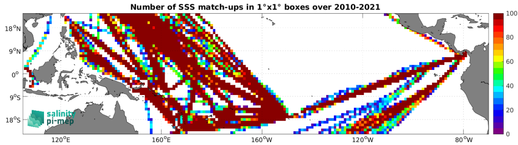
Figure 4: Number of SSS match-ups between TSG (LEGOS-DM) SSS and the SMOS SSS L3 v335 - 10 Days - 25 km (CATDS-CPDC) SSS product for the Tropical Pacific Ocean Pi-MEP region over 1^\circ \times 1^\circ boxes and for the full satellite product period.
