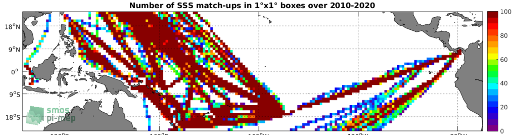
Figure 4: Number of SSS match-ups between TSG (LEGOS-DM) SSS and the SMOS SSS L3 v335 - 10 Days - 25 km (CATDS-CPDC) SSS product for the Tropical Pacific Ocean Pi-MEP region over 1^\circ \times 1^\circ boxes and for the full satellite product period.
