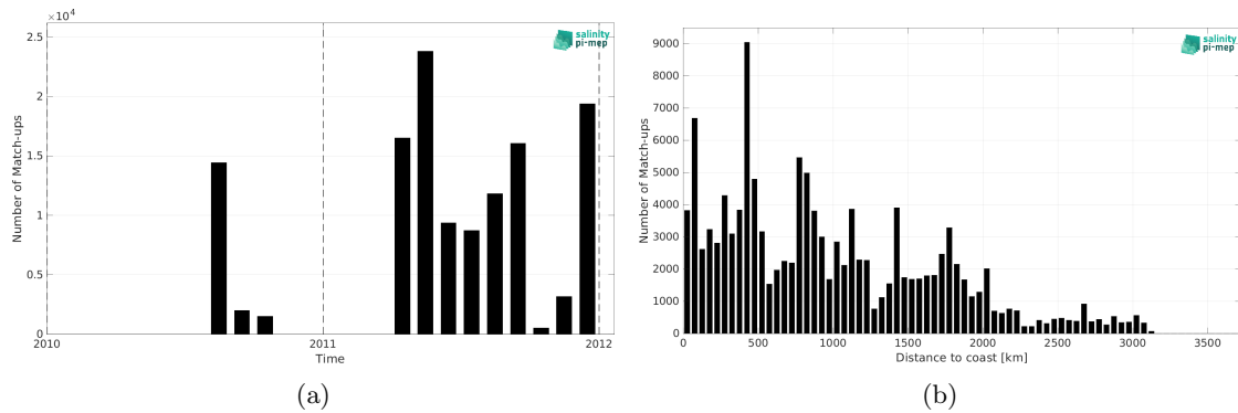
Figure 2: Number of match-ups between TSG (GOSUD-Sailing-ship) and SMOS SSS L3 v335 - 10 Days - 25 km (CATDS-CPDC) SSS as a function of time (a) and as function of the distance to coast (b) over the Tropical Pacific Ocean Pi-MEP region and for the full satellite product period.
