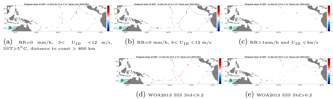
Figure 14: Temporal mean gridded over spatial boxes of size 1^\circ \times 1^\circ of \Delta SSS (SMOS SSS L3 v335 - 10 Days - 25 km (CATDS-CPDC) - TSG (GOSUD-Sailing-ship)) for 5 different subdatasets corresponding to:RR=0 mm/h, 3 < U_{10} < 12 m/s, SST > 5^\circ\text{C} , distance to coast > 800 km (a), RR=0 mm/h, 3 < U_{10} < 12 m/s (b), RR > 1 mm/h and U_{10} < 4 m/s (c), WOA2013 SSS Std < 0.2 (d), WOA2013 SSS Std > 0.2 (e).
