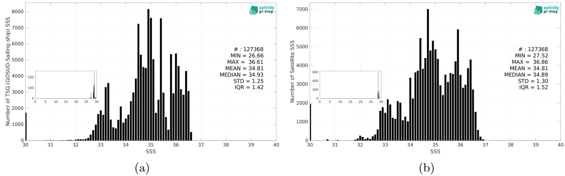
Figure 3: Histograms of SSS from TSG (GOSUD-Sailing-ship) (a) and SMOS SSS L3 v335 - 10 Days - 25 km (CATDS-CPDC) (b) considering all match-up pairs per bins of 0.1 over the Tropical Pacific Ocean Pi-MEP region and for the full satellite product period.
