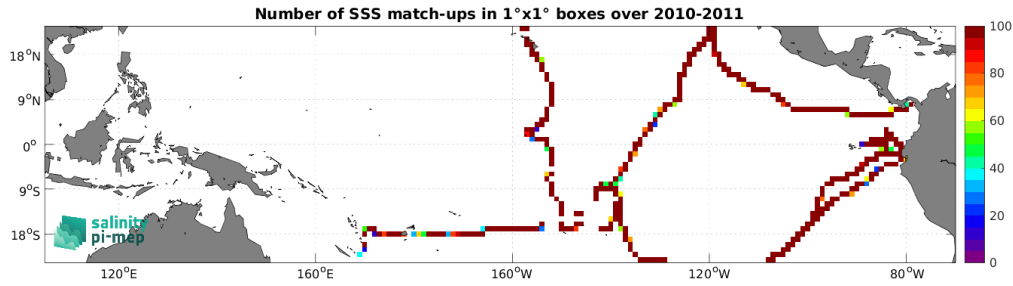
Figure 5: Number of SSS match-ups between TSG (GOSUD-Sailing-ship) SSS and the SMOS SSS L3 v335 - 10 Days - 25 km (CATDS-CPDC) SSS product for the Tropical Pacific Ocean Pi-MEP region over 1^\circ \times 1^\circ boxes and for the full satellite product period.
