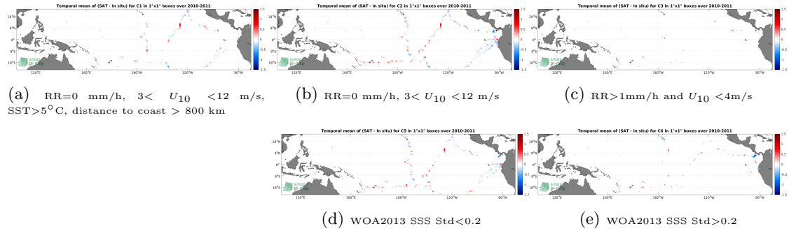
Figure 12: Temporal mean gridded over spatial boxes of size 1^{\circ}\times 1^{\circ} of \Delta SSS (SMOS SSS L3 v335 - 10 Days - 25 km (CATDS-CPDC) - TSG (GOSUD-Sailing-ship)) for 5 different subdatasets corresponding to:RR=0 mm/h, 3 < U_{10} < 12 m/s, SST >5^{\circ}\text{C} , distance to coast > 800 km (a), RR=0 mm/h, 3 < U_{10} < 12 m/s (b), RR >1 mm/h and U_{10} < 4 m/s (c), WOA2013 SSS Std <0.2 (d), WOA2013 SSS Std >0.2 (e).
