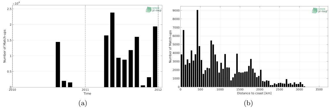
Figure 1: Number of match-ups between TSG (GOSUD-Sailing-ship) and SMOS SSS L3 v335 - 10 Days - 25 km (CATDS-CPDC) SSS as a function of time (a) and as function of the distance to coast (b) over the Tropical Pacific Ocean Pi-MEP region and for the full satellite product period.
