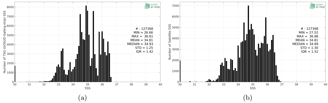
Figure 2: Histograms of SSS from TSG (GOSUD-Sailing-ship) (a) and SMOS SSS L3 v335 - 10 Days - 25 km (CATDS-CPDC) (b) considering all match-up pairs per bins of 0.1 over the Tropical Pacific Ocean Pi-MEP region and for the full satellite product period.
