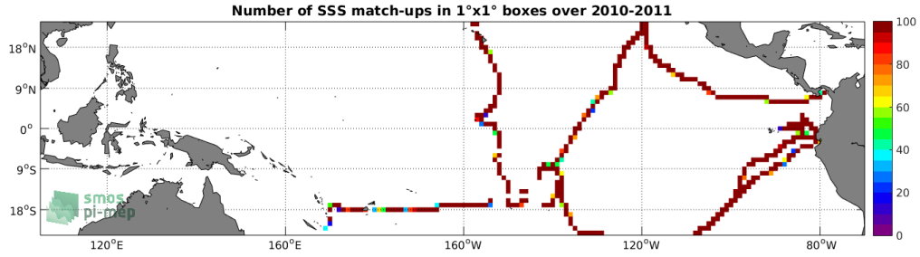
Figure 4: Number of SSS match-ups between TSG (GOSUD-Sailing-ship) SSS and the SMOS SSS L3 v335 - 10 Days - 25 km (CATDS-CPDC) SSS product for the Tropical Pacific Ocean Pi-MEP region over 1^\circ \times 1^\circ boxes and for the full satellite product period.
