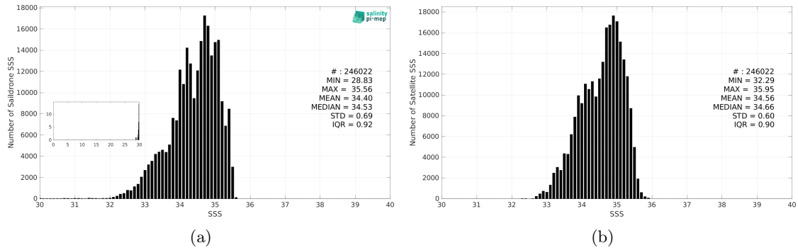
Figure 3: Histograms of SSS from Saildrone (a) and SMOS SSS L3 v335 - 10 Days - 25 km (CATDS-CPDC) (b) considering all match-up pairs per bins of 0.1 over the Tropical Pacific Ocean Pi-MEP region and for the full satellite product period.
