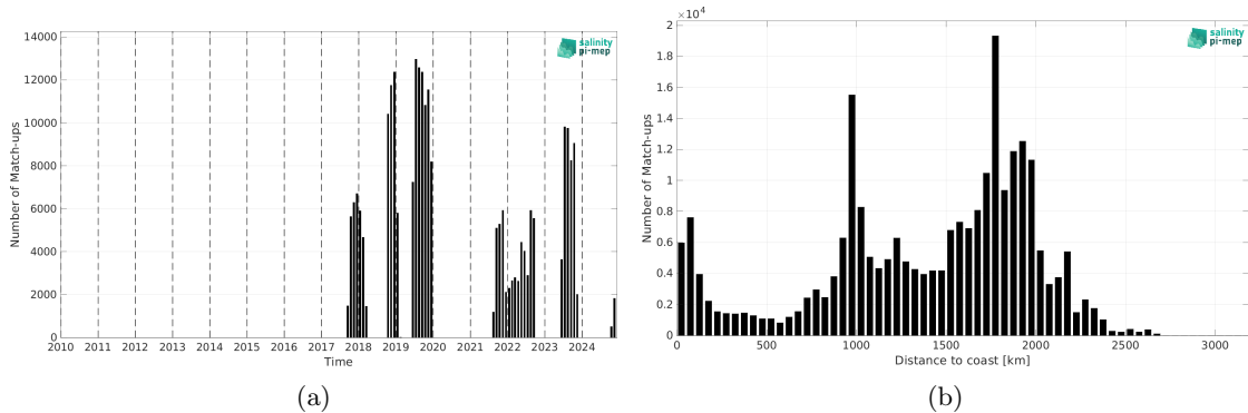
Figure 2: Number of match-ups between Saildrone and SMOS SSS L3 v335 - 10 Days - 25 km (CATDS-CPDC) SSS as a function of time (a) and as function of the distance to coast (b) over the Tropical Pacific Ocean Pi-MEP region and for the full satellite product period.
