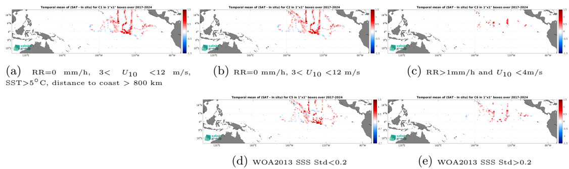
Figure 14: Temporal mean gridded over spatial boxes of size 1^\circ \times 1^\circ of \Delta SSS (SMOS SSS L3 v335 - 10 Days - 25 km (CATDS-CPDC) - Saildrone) for 5 different subdatasets corresponding to: RR=0 mm/h, 3 < U_{10} < 12 m/s, SST > 5^\circ\text{C} , distance to coast > 800 km (a), RR=0 mm/h, 3 < U_{10} < 12 m/s (b), RR > 1 mm/h and U_{10} < 4 m/s (c), WOA2013 SSS Std < 0.2 (d), WOA2013 SSS Std > 0.2 (e).
