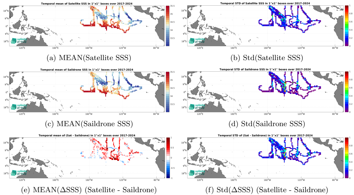
Figure 7: Temporal mean (left) and Std (right) of SSS from SMOS SSS L3 v335 - 10 Days - 25 km (CATDS-CPDC) (top), Saildrone (middle), and of \Delta SSS (Satellite - Saildrone). Only match-up pairs are used to generate these maps.
