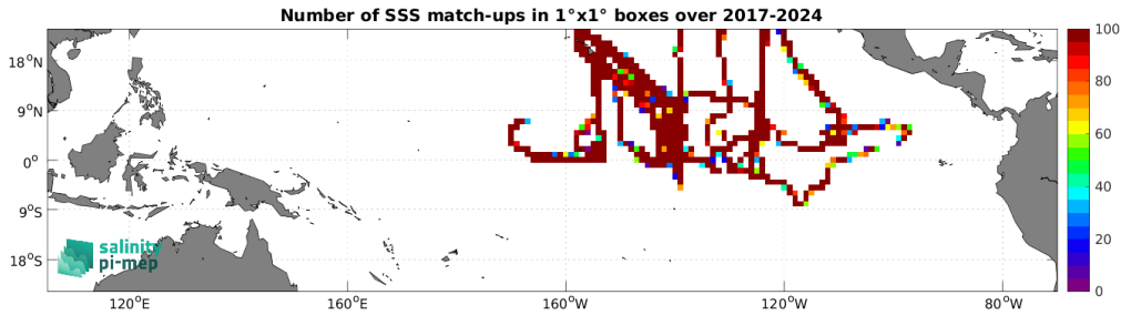
Figure 5: Number of SSS match-ups between Saildrone SSS and the SMOS SSS L3 v335 - 10 Days - 25 km (CATDS-CPDC) SSS product for the Tropical Pacific Ocean Pi-MEP region over 1^\circ \times 1^\circ boxes and for the full satellite product period.
