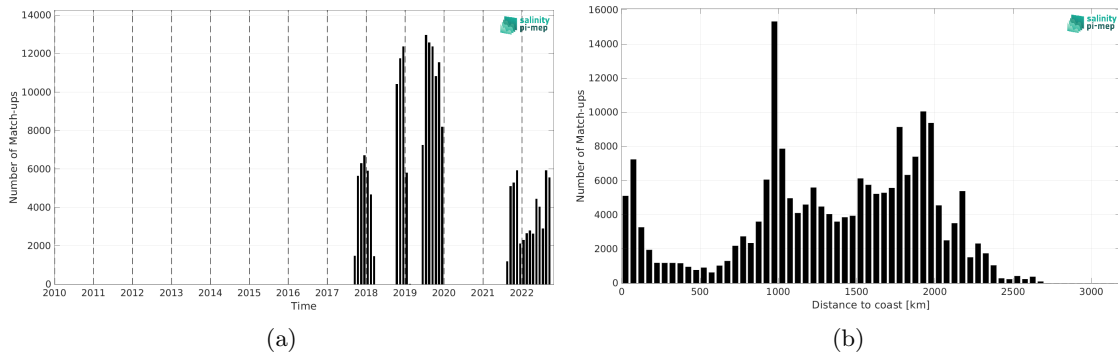
Figure 2: Number of match-ups between Saildrone and SMOS SSS L3 v335 - 10 Days - 25 km (CATDS-CPDC) SSS as a function of time (a) and as function of the distance to coast (b) over the Tropical Pacific Ocean Pi-MEP region and for the full satellite product period.
