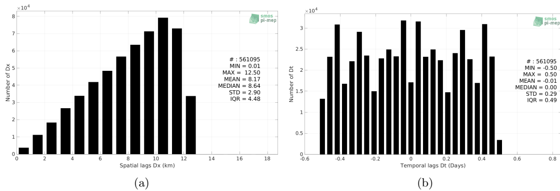
Figure 4: Histograms of the spatial (a) and temporal (b) lags between the location/time of the Surface drifters measurement and the date of the corresponding SMOS SSS L3 v335 - 10 Days - 25 km (CATDS-CPDC) SSS pixel.
