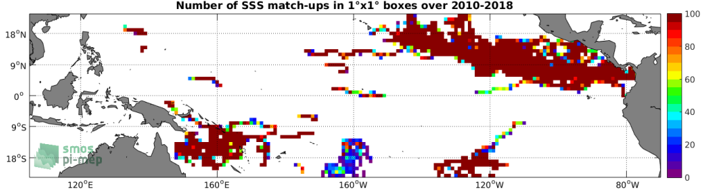
Figure 3: Number of SSS match-ups between Surface drifters SSS and the SMOS SSS L3 v335 - 10 Days - 25 km (CATDS-CPDC) SSS product for the Tropical Pacific Ocean Pi-MEP region over 1^\circ \times 1^\circ boxes and for the full satellite product period.
