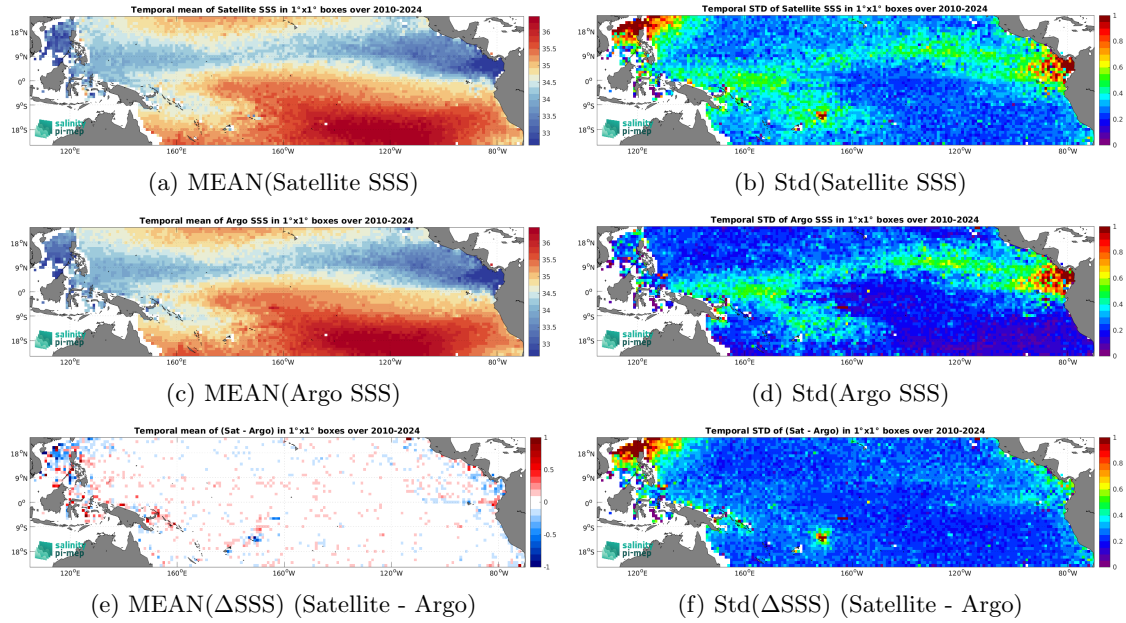
Figure 7: Temporal mean (left) and Std (right) of SSS from SMOS SSS L3 v335 - 10 Days - 25 km (CATDS-CPDC) (top), Argo (middle), and of \Delta SSS (Satellite - Argo). Only match-up pairs are used to generate these maps.
