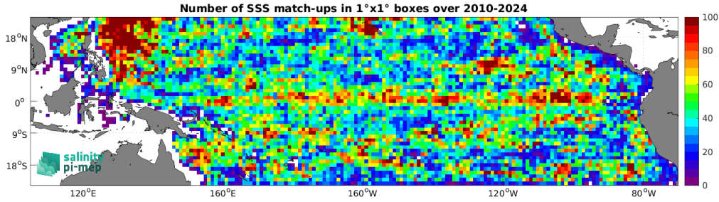
Figure 5: Number of SSS match-ups between Argo SSS and the SMOS SSS L3 v335 - 10 Days - 25 km (CATDS-CPDC) SSS product for the Tropical Pacific Ocean Pi-MEP region over 1^\circ \times 1^\circ boxes and for the full satellite product period.
