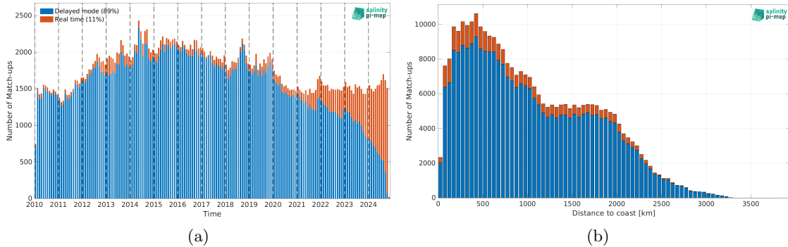
Figure 2: Number of match-ups between Argo and SMOS SSS L3 v335 - 10 Days - 25 km (CATDS-CPDC) SSS as a function of time (a) and as function of the distance to coast (b) over the Tropical Pacific Ocean Pi-MEP region and for the full satellite product period.
