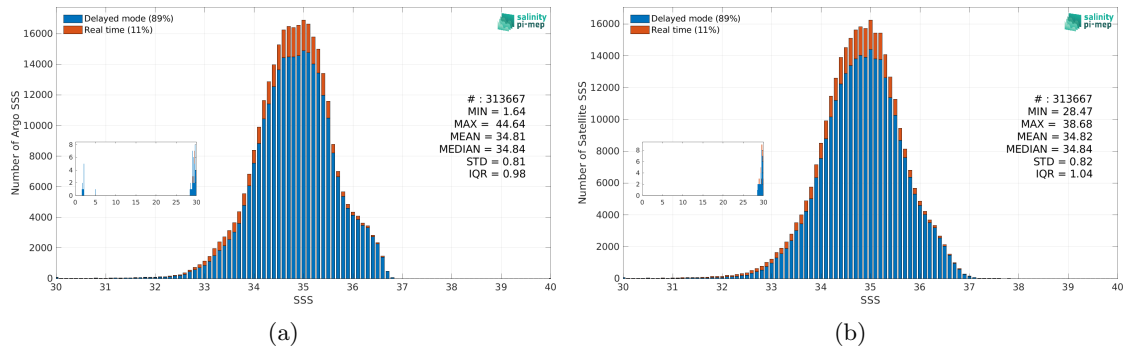
Figure 3: Histograms of SSS from Argo (a) and SMOS SSS L3 v335 - 10 Days - 25 km (CATDS-CPDC) (b) considering all match-up pairs per bins of 0.1 over the Tropical Pacific Ocean Pi-MEP region and for the full satellite product period.
