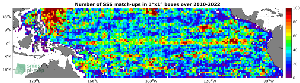
Figure 4: Number of SSS match-ups between Argo SSS and the SMOS SSS L3 v335 - 10 Days - 25 km (CATDS-CPDC) SSS product for the Tropical Pacific Ocean Pi-MEP region over 1^\circ \times 1^\circ boxes and for the full satellite product period.
