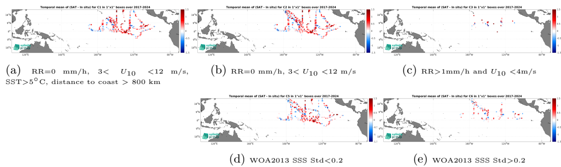
Figure 14: Temporal mean gridded over spatial boxes of size 1^\circ \times 1^\circ of \Delta SSS (SMOS SSS L2Q v333 - 0.25 Deg (CATDS-CPDC) - Saildrone) for 5 different subdatasets corresponding to:RR=0 mm/h, 3 < U_{10} < 12 m/s, SST>5°C, distance to coast > 800 km (a), RR=0 mm/h, 3 < U_{10} < 12 m/s (b), RR>1mm/h and U_{10} < 4 m/s (c), WOA2013 SSS Std<0.2 (d), WOA2013 SSS Std>0.2 (e).
