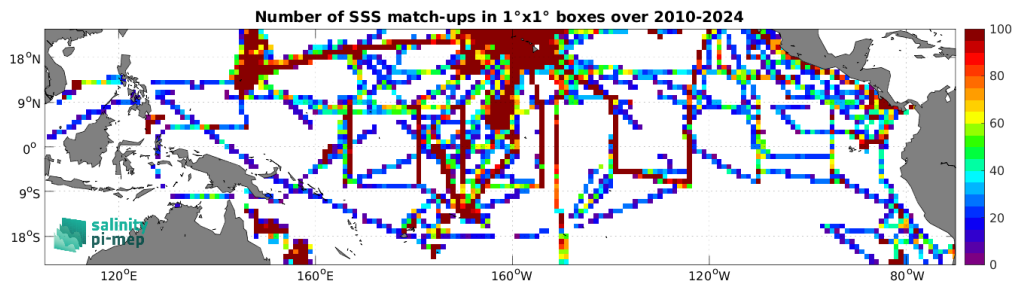
Figure 5: Number of SSS match-ups between TSG (SAMOS) SSS and the SMOS SSS L3 v332 - 9 Days (CATDS-CPDC) SSS product for the Tropical Pacific Ocean Pi-MEP region over 1^\circ \times 1^\circ boxes and for the full satellite product period.
