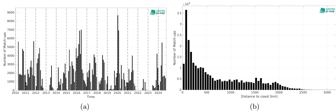
Figure 2: Number of match-ups between TSG (SAMOS) and SMOS SSS L3 v332 - 9 Days (CATDS-CPDC) SSS as a function of time (a) and as function of the distance to coast (b) over the Tropical Pacific Ocean Pi-MEP region and for the full satellite product period.
