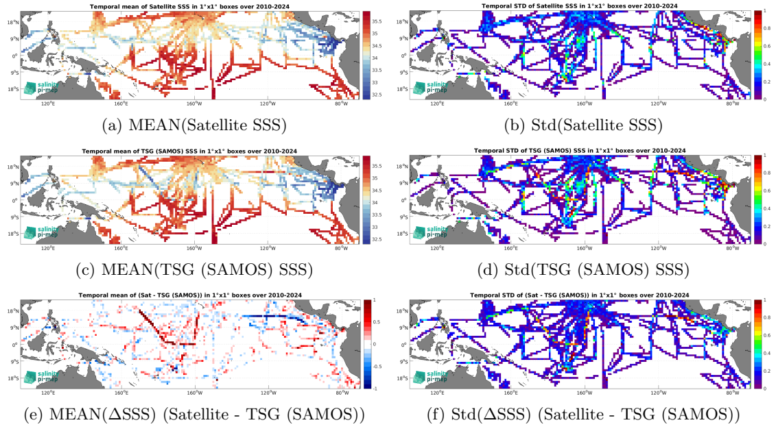
Figure 7: Temporal mean (left) and Std (right) of SSS from SMOS SSS L3 v332 - 9 Days (CATDS-CPDC) (top), TSG (SAMOS) (middle), and of \Delta SSS (Satellite - TSG (SAMOS)). Only match-up pairs are used to generate these maps.
