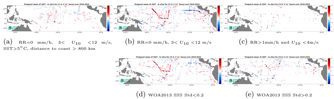
Figure 14: Temporal mean gridded over spatial boxes of size 1^\circ \times 1^\circ of \Delta SSS (SMOS SSS L3 v332 - 9 Days (CATDS-CPDC) - TSG (SAMOS)) for 5 different subdatasets corresponding to:RR=0 mm/h, 3 < U_{10} < 12 m/s, SST > 5^\circ\text{C} , distance to coast > 800 km (a), RR=0 mm/h, 3 < U_{10} < 12 m/s (b), RR > 1 mm/h and U_{10} < 4 m/s (c), WOA2013 SSS Std < 0.2 (d), WOA2013 SSS Std > 0.2 (e).
