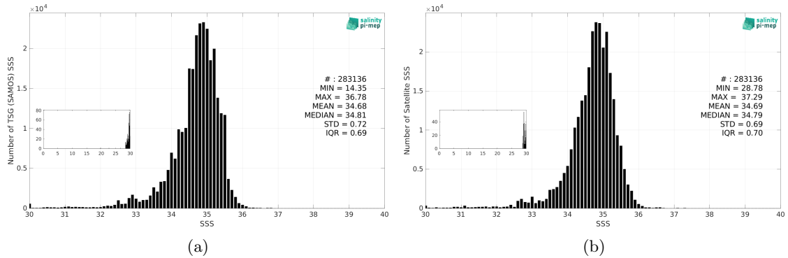
Figure 3: Histograms of SSS from TSG (SAMOS) (a) and SMOS SSS L3 v332 - 9 Days (CATDS-CPDC) (b) considering all match-up pairs per bins of 0.1 over the Tropical Pacific Ocean Pi-MEP region and for the full satellite product period.
