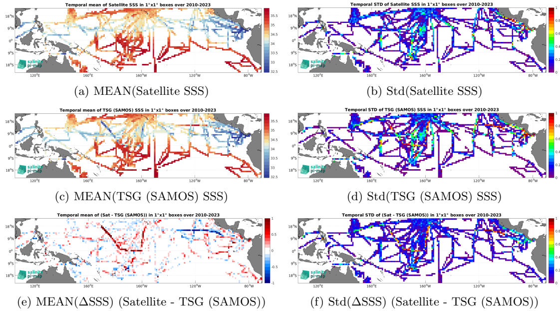
Figure 6: Temporal mean (left) and Std (right) of SSS from SMOS SSS L3 v332 - 9 Days (CATDS-CPDC) (top), TSG (SAMOS) (middle), and of \Delta SSS (Satellite - TSG (SAMOS)). Only match-up pairs are used to generate these maps.
