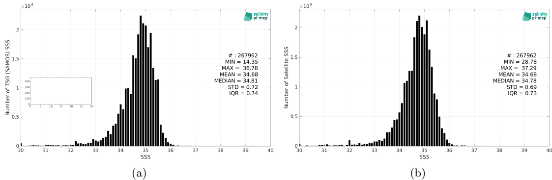
Figure 2: Histograms of SSS from TSG (SAMOS) (a) and SMOS SSS L3 v332 - 9 Days (CATDS-CPDC) (b) considering all match-up pairs per bins of 0.1 over the Tropical Pacific Ocean Pi-MEP region and for the full satellite product period.
