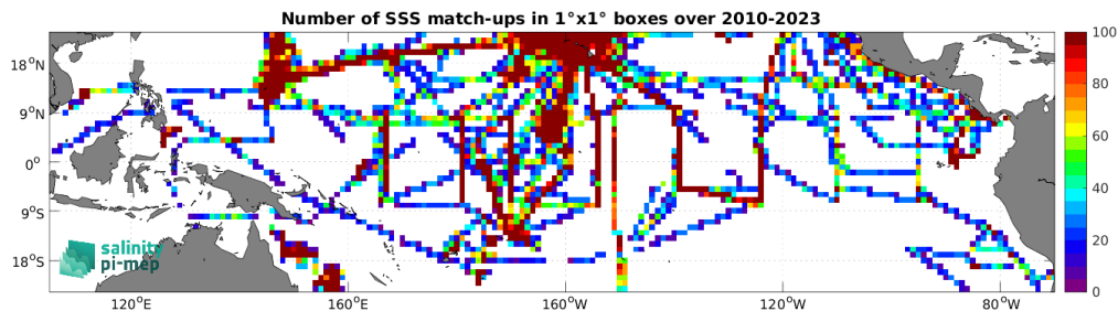
Figure 4: Number of SSS match-ups between TSG (SAMOS) SSS and the SMOS SSS L3 v332 - 9 Days (CATDS-CPDC) SSS product for the Tropical Pacific Ocean Pi-MEP region over 1^\circ \times 1^\circ boxes and for the full satellite product period.
