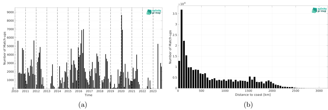
Figure 1: Number of match-ups between TSG (SAMOS) and SMOS SSS L3 v332 - 9 Days (CATDS-CPDC) SSS as a function of time (a) and as function of the distance to coast (b) over the Tropical Pacific Ocean Pi-MEP region and for the full satellite product period.
